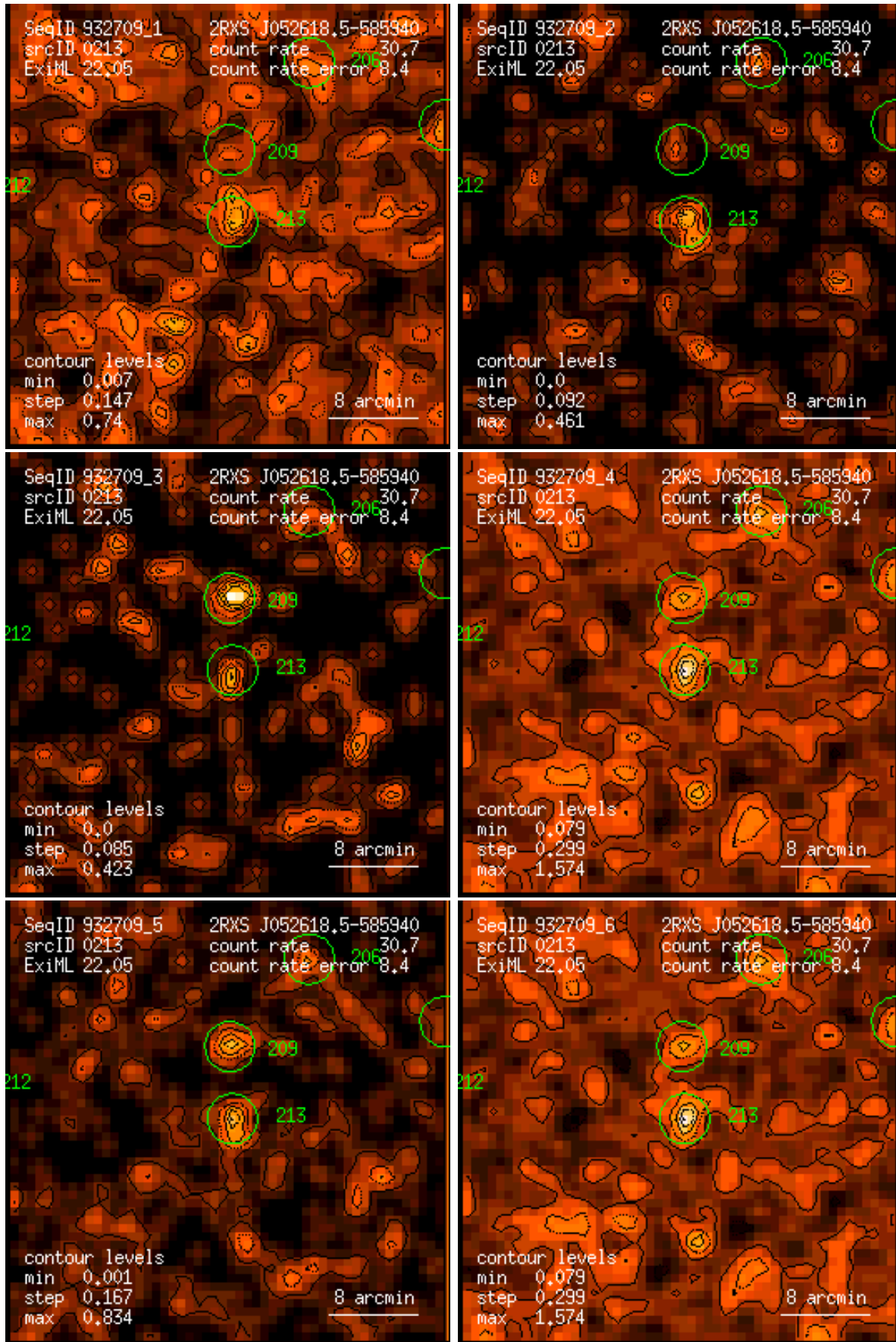
Figure 213: RASS 932709: detection 0213: band rate images, Gaussian filter: (1) PSPC channels 11 – 41, (2) 52 – 90, (3) 91 – 201, (4) 11 – 235, (5) 52 – 201, (6) 11 – 201. Broad band rates in counts/ks. Band rate contour levels in counts/ks/arcmin 2 .
