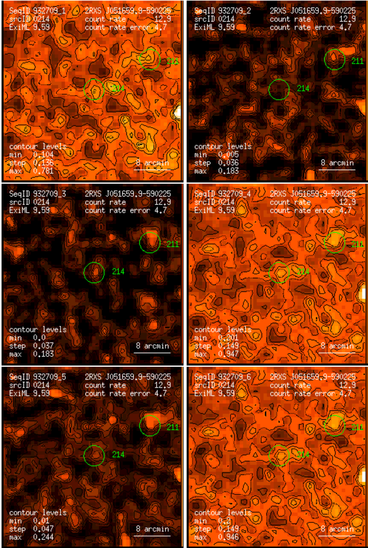
Figure 214: RASS 932709: detection 0214: band rate images, Gaussian filter: (1) PSPC channels 11 – 41, (2) 52 – 90, (3) 91 – 201, (4) 11 – 235, (5) 52 – 201, (6) 11 – 201. Broad band rates in counts/ks. Band rate contour levels in counts/ks/arcmin 2 .
