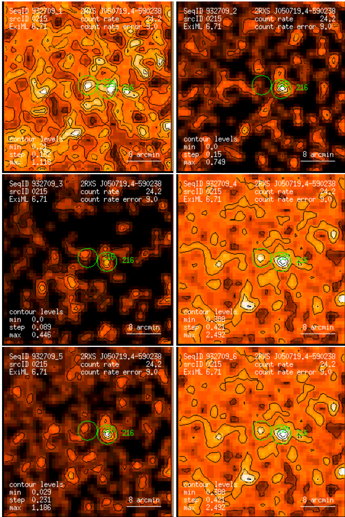
Figure 215: RASS 932709: detection 0215: band rate images, Gaussian filter: (1) PSPC channels 11 – 41, (2) 52 – 90, (3) 91 – 201, (4) 11 – 235, (5) 52 – 201, (6) 11 – 201. Broad band rates in counts/ks. Band rate contour levels in counts/ks/arcmin 2 .
