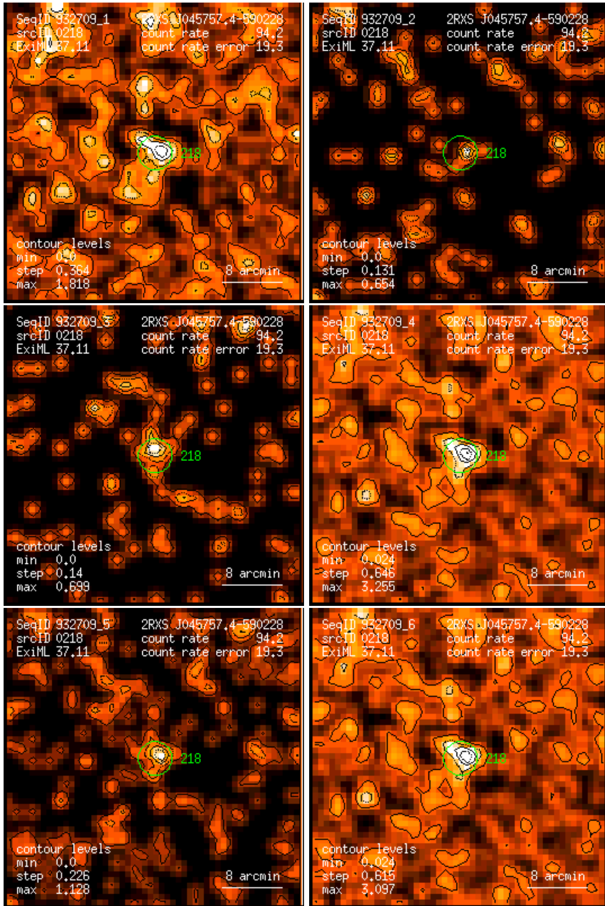
Figure 218: RASS 932709: detection 0218: band rate images, Gaussian filter: (1) PSPC channels 11 – 41, (2) 52 – 90, (3) 91 – 201, (4) 11 – 235, (5) 52 – 201, (6) 11 – 201. Broad band rates in counts/ks. Band rate contour levels in counts/ks/arcmin 2 .
