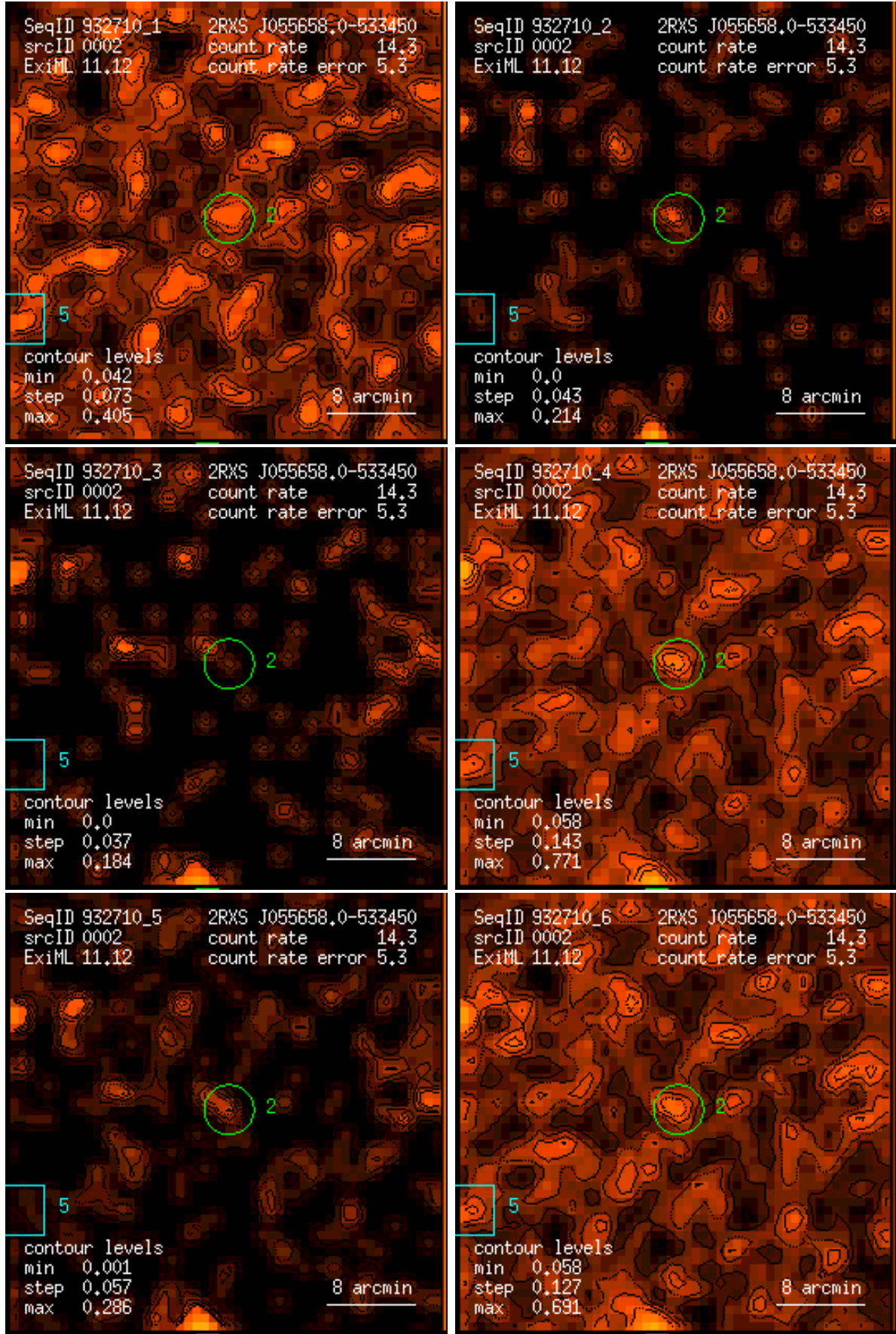
Figure 2: RASS 932710: detection 0002: band rate images, Gaussian filter: (1) PSPC channels 11 – 41, (2) 52 – 90, (3) 91 – 201, (4) 11 – 235, (5) 52 – 201, (6) 11 – 201. Broad band rates in counts/ks. Band rate contour levels in counts/ks/arcmin 2 .
