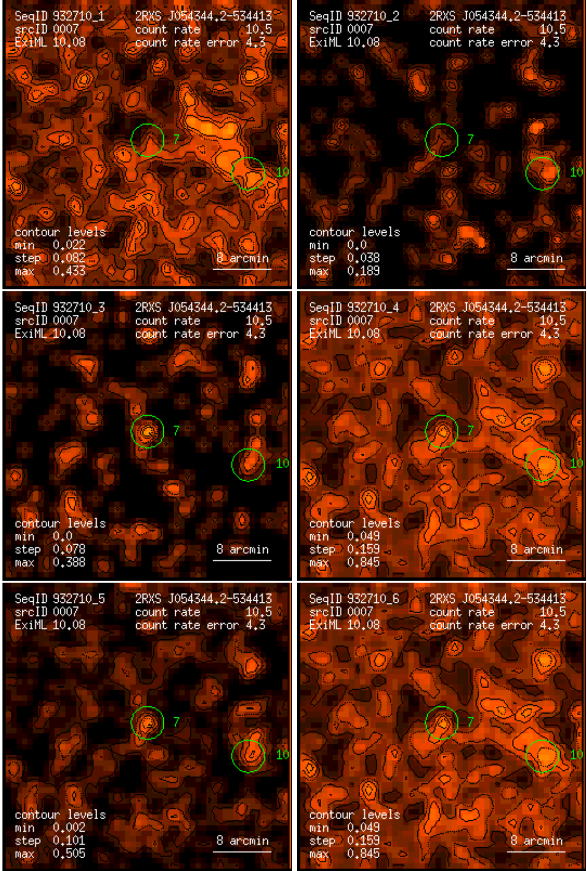
Figure 7: RASS 932710: detection 0007: band rate images, Gaussian filter: (1) PSPC channels 11 – 41, (2) 52 – 90, (3) 91 – 201, (4) 11 – 235, (5) 52 – 201, (6) 11 – 201. Broad band rates in counts/ks. Band rate contour levels in counts/ks/arcmin 2 .
