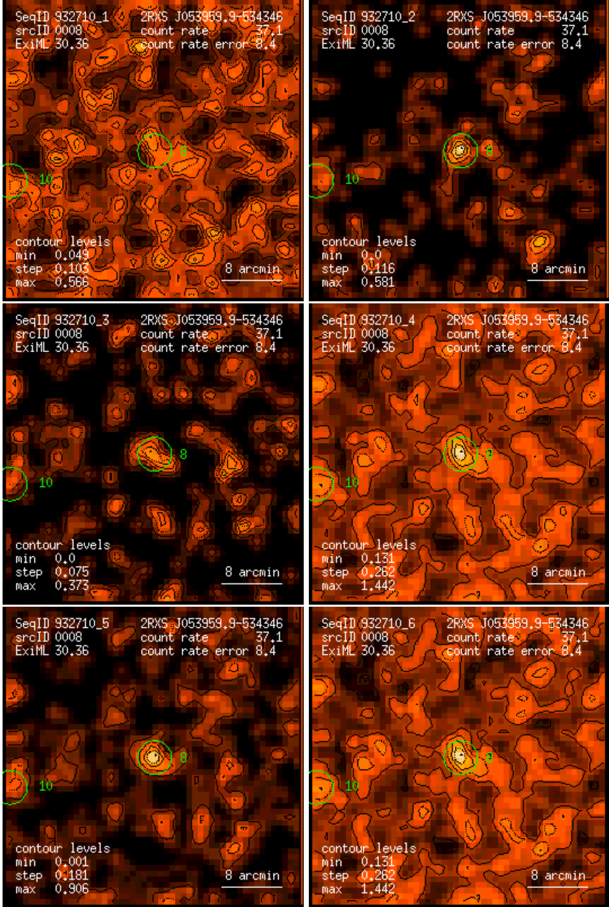
Figure 8: RASS 932710: detection 0008: band rate images, Gaussian filter: (1) PSPC channels 11 – 41, (2) 52 – 90, (3) 91 – 201, (4) 11 – 235, (5) 52 – 201, (6) 11 – 201. Broad band rates in counts/ks. Band rate contour levels in counts/ks/arcmin 2 .
