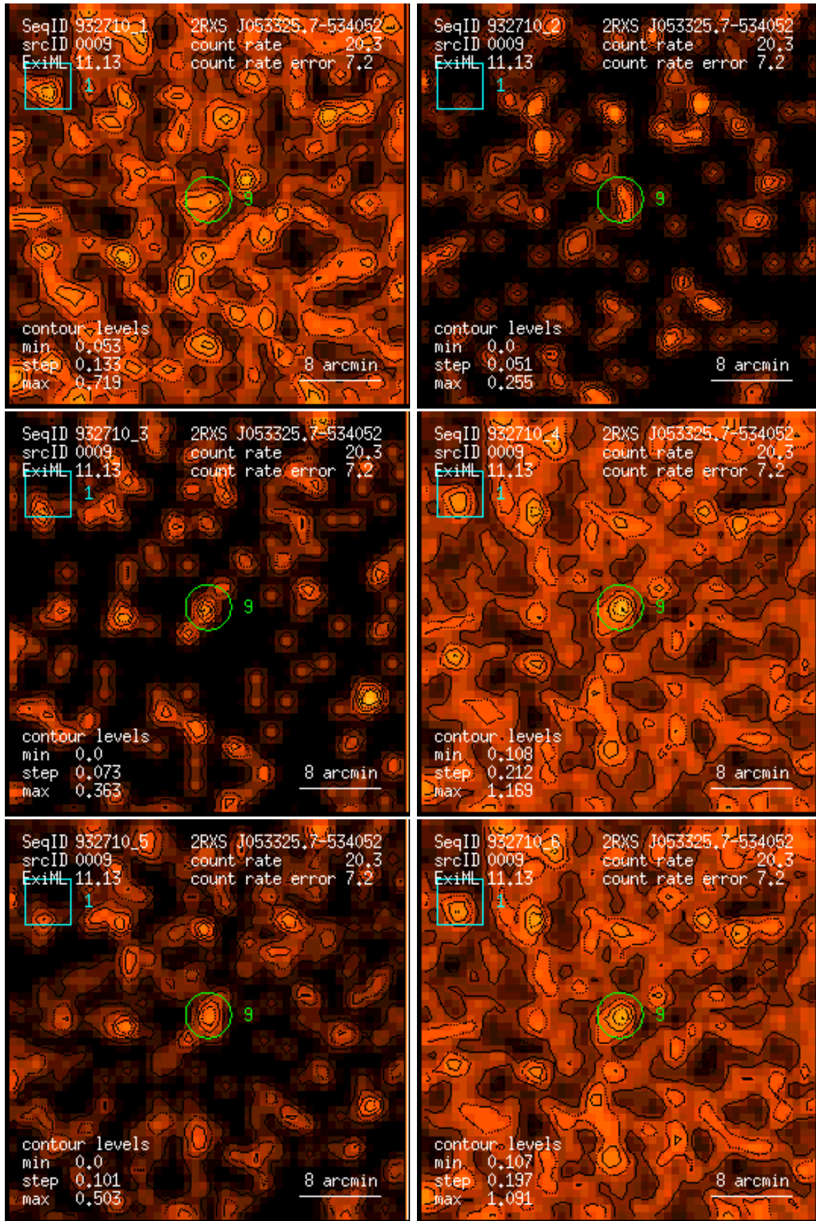
Figure 9: RASS 932710: detection 0009: band rate images, Gaussian filter: (1) PSPC channels 11 – 41, (2) 52 – 90, (3) 91 – 201, (4) 11 – 235, (5) 52 – 201, (6) 11 – 201. Broad band rates in counts/ks. Band rate contour levels in counts/ks/arcmin 2 .
