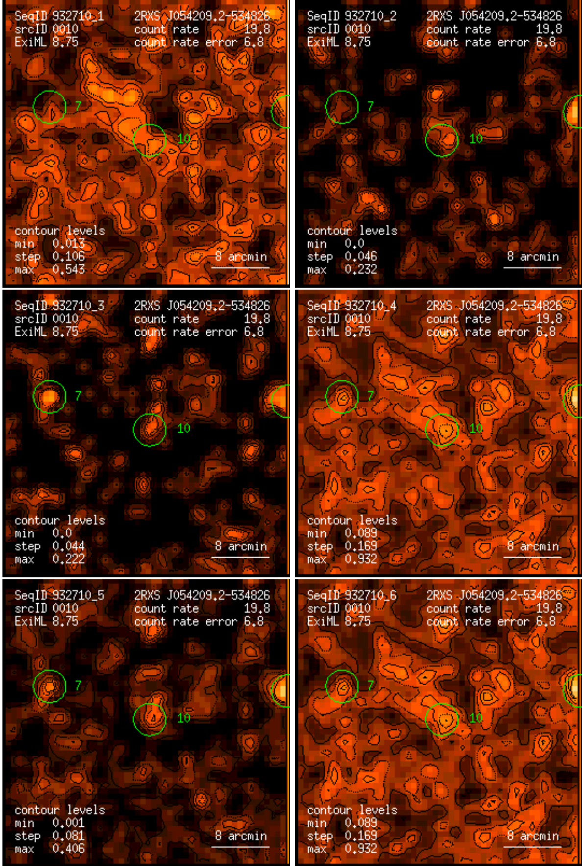
Figure 10: RASS 932710: detection 0010: band rate images, Gaussian filter: (1) PSPC channels 11 – 41, (2) 52 – 90, (3) 91 – 201, (4) 11 – 235, (5) 52 – 201, (6) 11 – 201. Broad band rates in counts/ks. Band rate contour levels in counts/ks/arcmin 2 .
