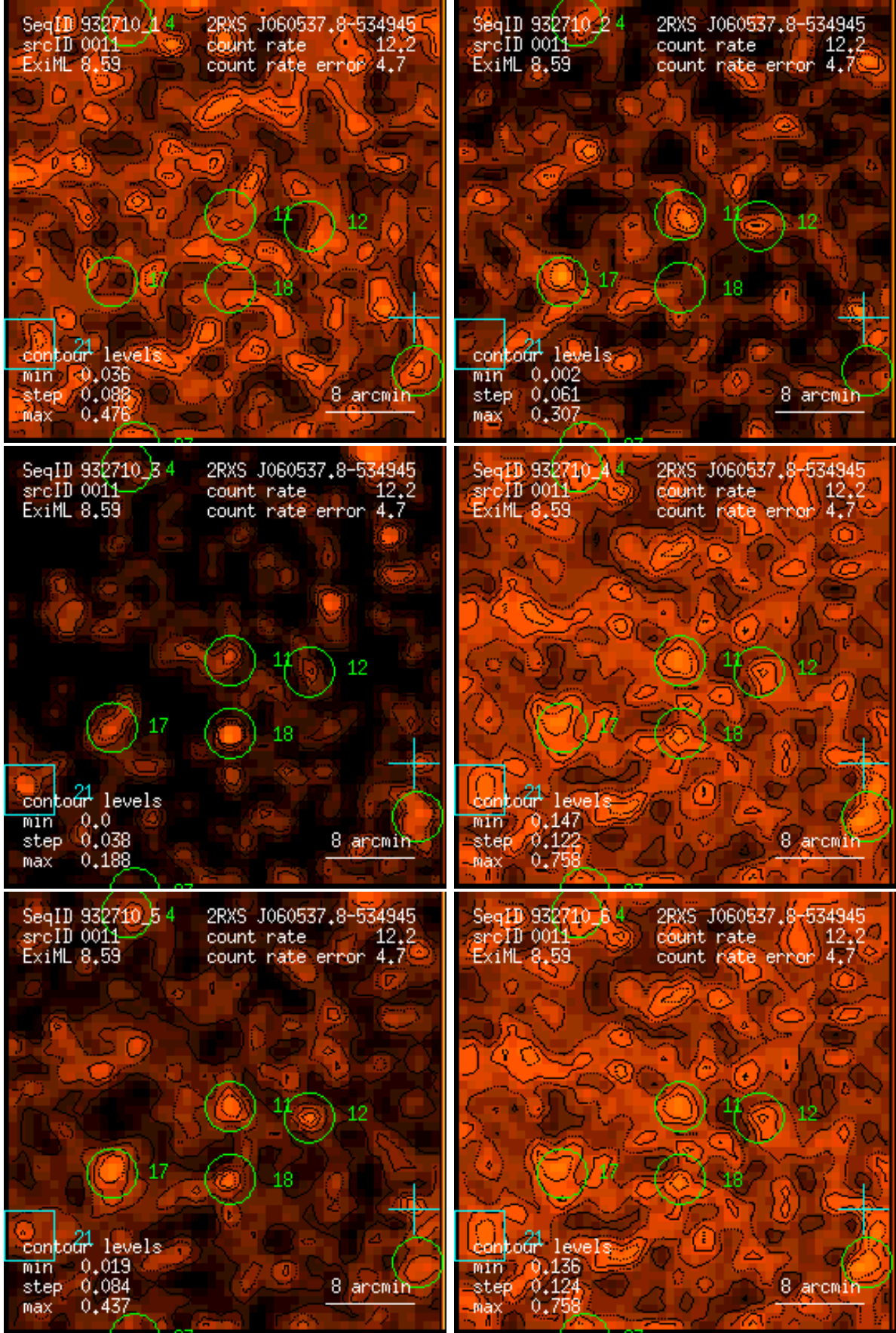
Figure 11: RASS 932710: detection 0011: band rate images, Gaussian filter: (1) PSPC channels 11 – 41, (2) 52 – 90, (3) 91 – 201, (4) 11 – 235, (5) 52 – 201, (6) 11 – 201. Broad band rates in counts/ks. Band rate contour levels in counts/ks/arcmin 2 .
