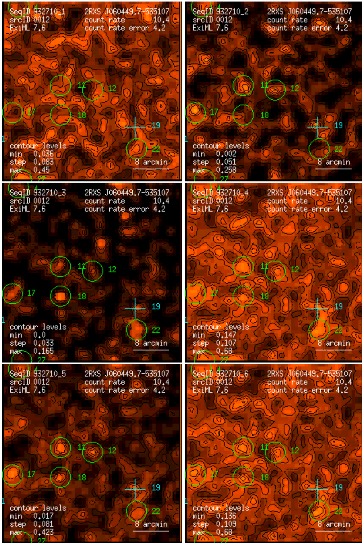
Figure 12: RASS 932710: detection 0012: band rate images, Gaussian filter: (1) PSPC channels 11 – 41, (2) 52 – 90, (3) 91 – 201, (4) 11 – 235, (5) 52 – 201, (6) 11 – 201. Broad band rates in counts/ks. Band rate contour levels in counts/ks/arcmin 2 .
