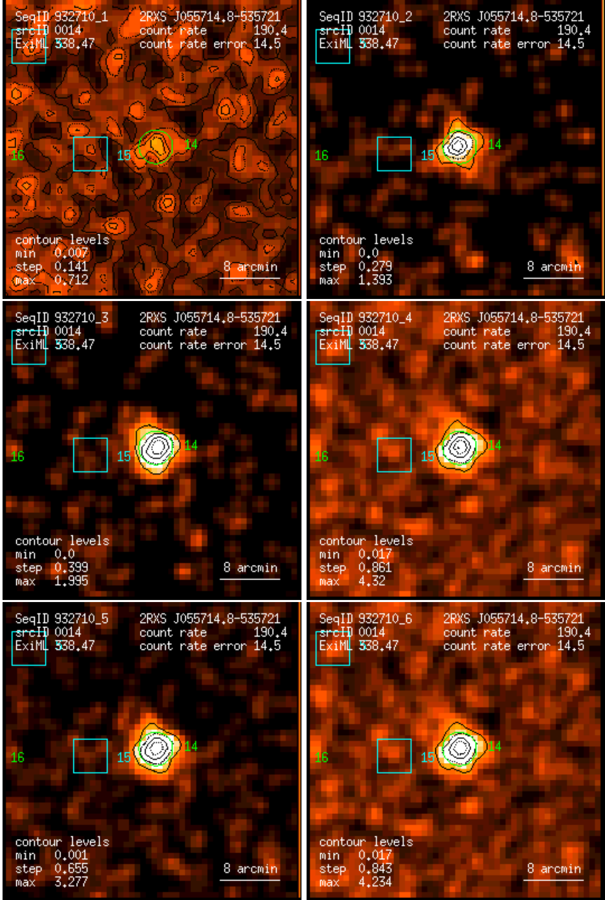
Figure 14: RASS 932710: detection 0014: band rate images, Gaussian filter: (1) PSPC channels 11 – 41, (2) 52 – 90, (3) 91 – 201, (4) 11 – 235, (5) 52 – 201, (6) 11 – 201. Broad band rates in counts/ks. Band rate contour levels in counts/ks/arcmin 2 .
