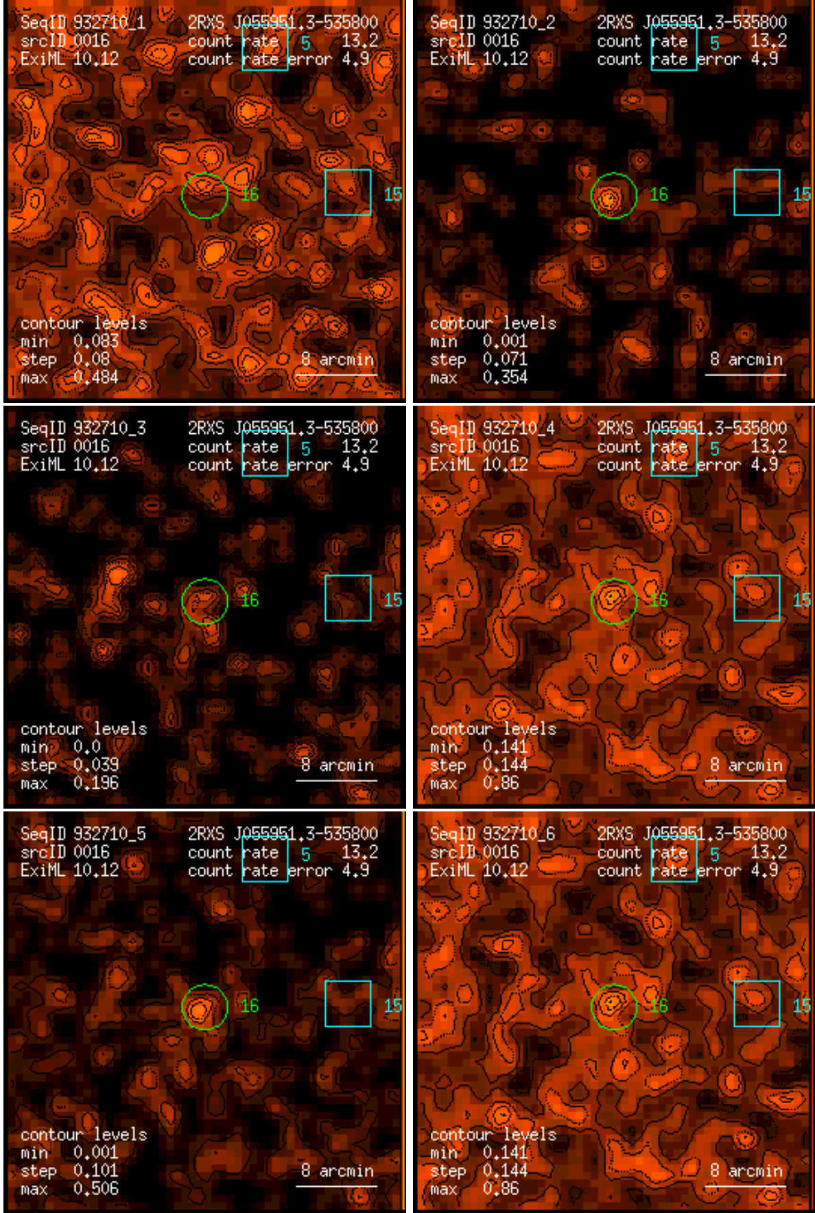
Figure 16: RASS 932710: detection 0016: band rate images, Gaussian filter: (1) PSPC channels 11 – 41, (2) 52 – 90, (3) 91 – 201, (4) 11 – 235, (5) 52 – 201, (6) 11 – 201. Broad band rates in counts/ks. Band rate contour levels in counts/ks/arcmin 2 .
