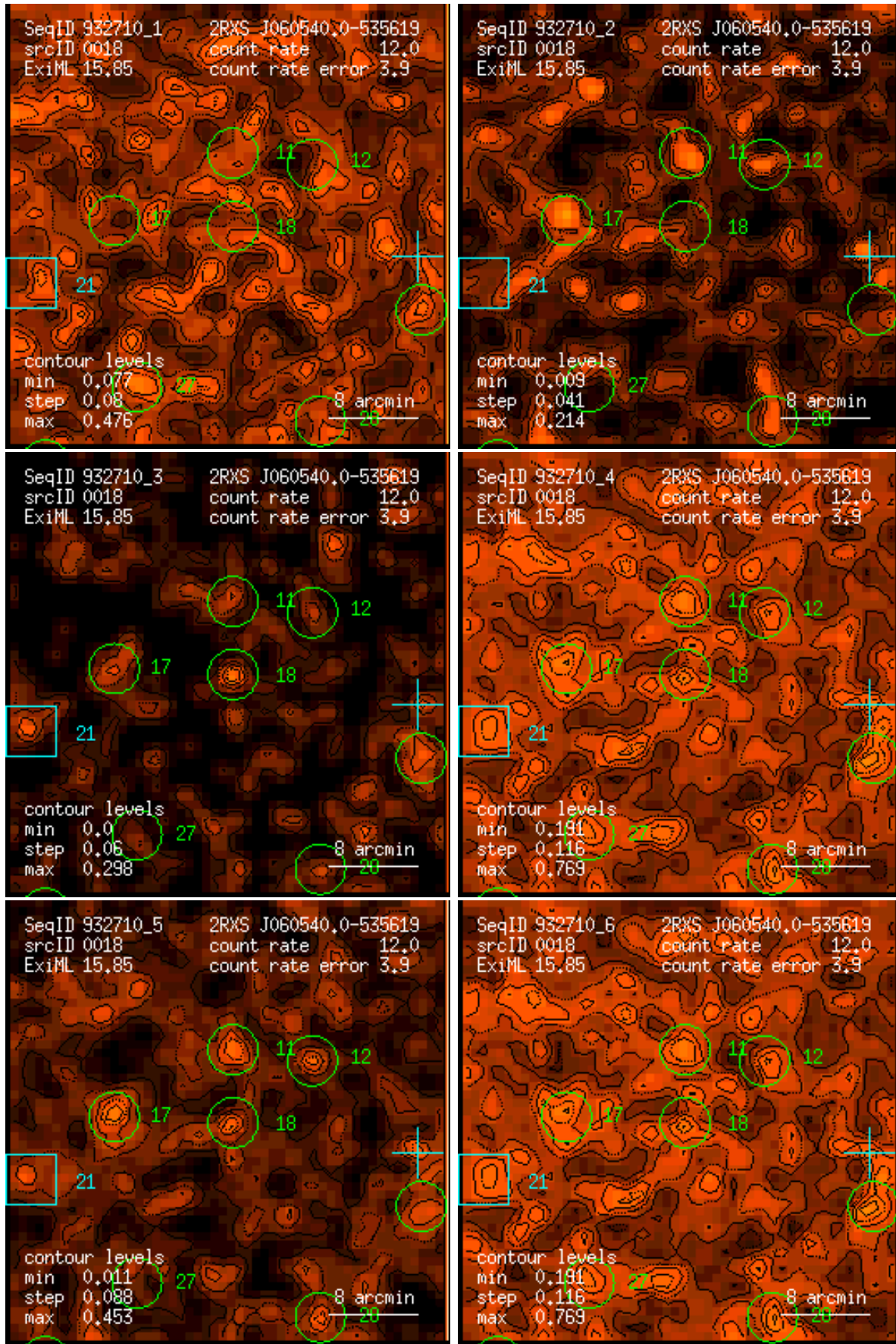
Figure 18: RASS 932710: detection 0018: band rate images, Gaussian filter: (1) PSPC channels 11 – 41, (2) 52 – 90, (3) 91 – 201, (4) 11 – 235, (5) 52 – 201, (6) 11 – 201. Broad band rates in counts/ks. Band rate contour levels in counts/ks/arcmin 2 .
