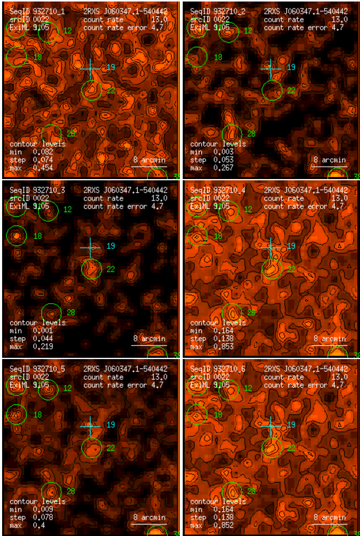
Figure 22: RASS 932710: detection 0022: band rate images, Gaussian filter: (1) PSPC channels 11 – 41, (2) 52 – 90, (3) 91 – 201, (4) 11 – 235, (5) 52 – 201, (6) 11 – 201. Broad band rates in counts/ks. Band rate contour levels in counts/ks/arcmin 2 .
