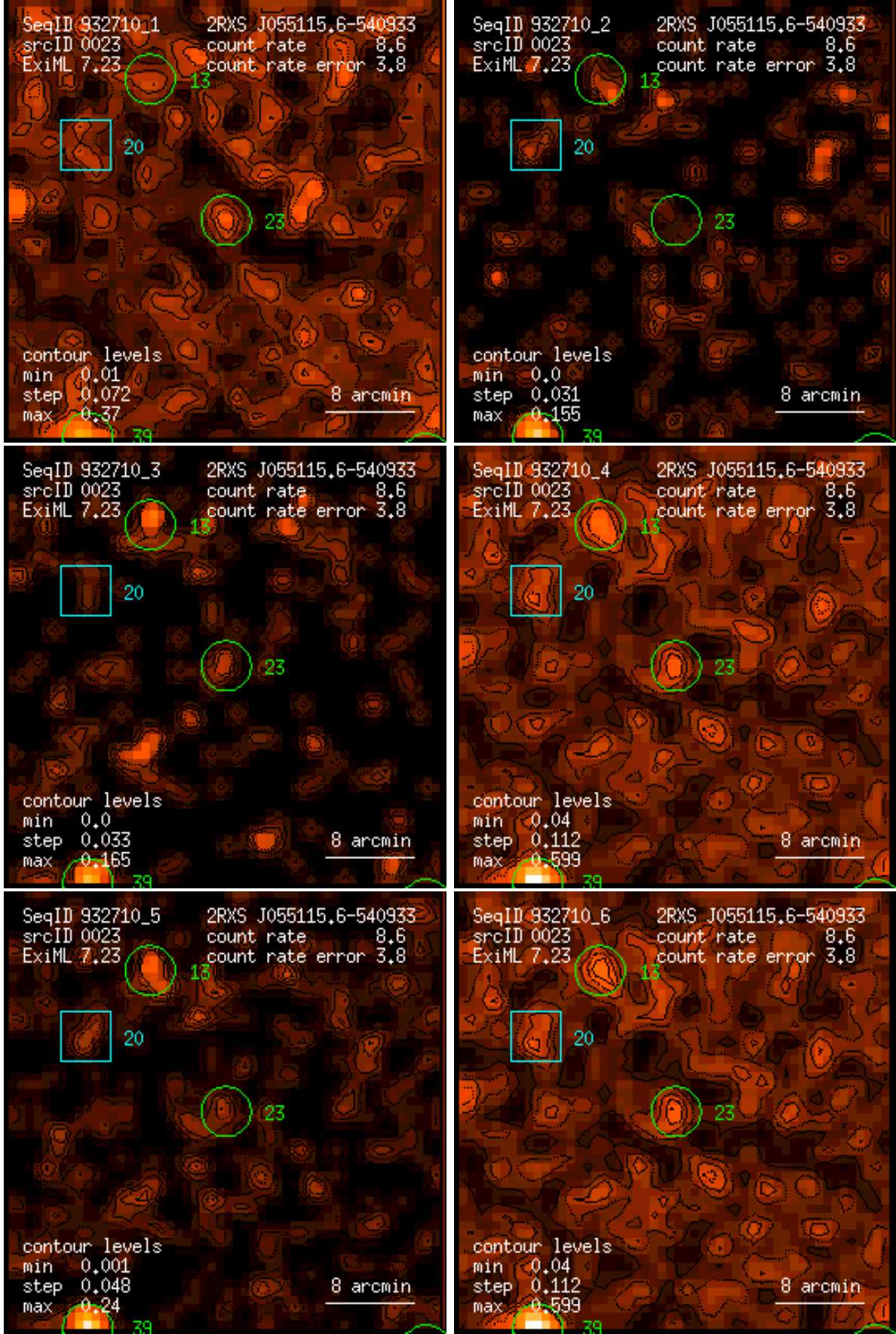
Figure 23: RASS 932710: detection 0023: band rate images, Gaussian filter: (1) PSPC channels 11 – 41, (2) 52 – 90, (3) 91 – 201, (4) 11 – 235, (5) 52 – 201, (6) 11 – 201. Broad band rates in counts/ks. Band rate contour levels in counts/ks/arcmin 2 .
