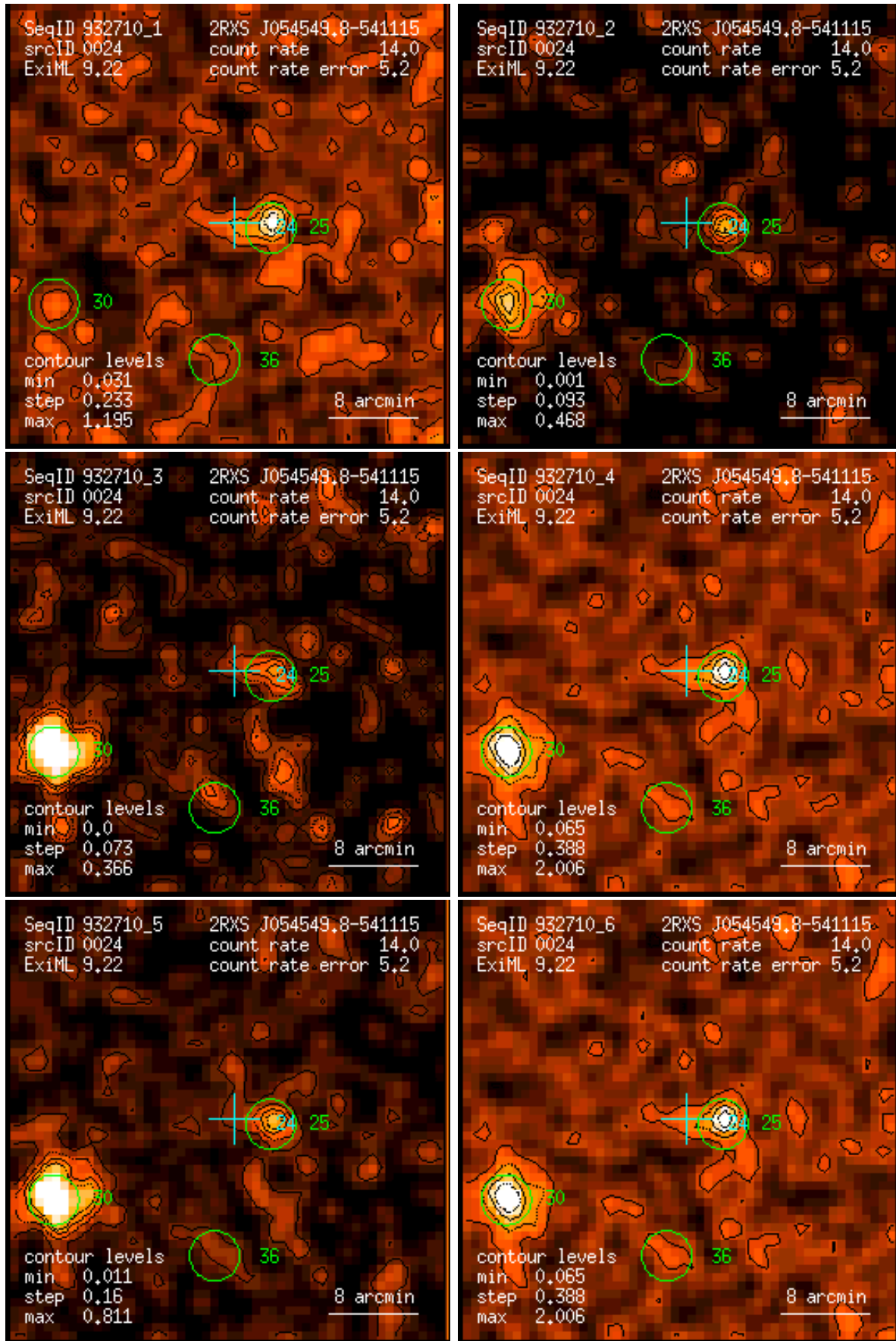
Figure 24: RASS 932710: detection 0024: band rate images, Gaussian filter: (1) PSPC channels 11 – 41, (2) 52 – 90, (3) 91 – 201, (4) 11 – 235, (5) 52 – 201, (6) 11 – 201. Broad band rates in counts/ks. Band rate contour levels in counts/ks/arcmin 2 .
