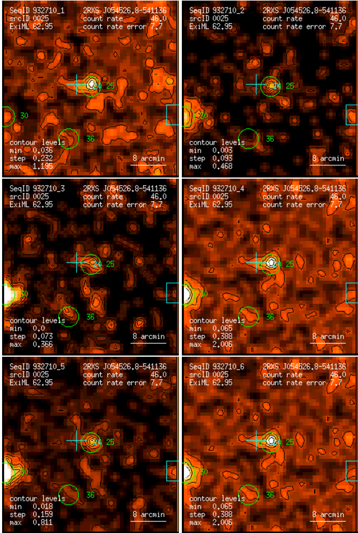
Figure 25: RASS 932710: detection 0025: band rate images, Gaussian filter: (1) PSPC channels 11 – 41, (2) 52 – 90, (3) 91 – 201, (4) 11 – 235, (5) 52 – 201, (6) 11 – 201. Broad band rates in counts/ks. Band rate contour levels in counts/ks/arcmin 2 .
