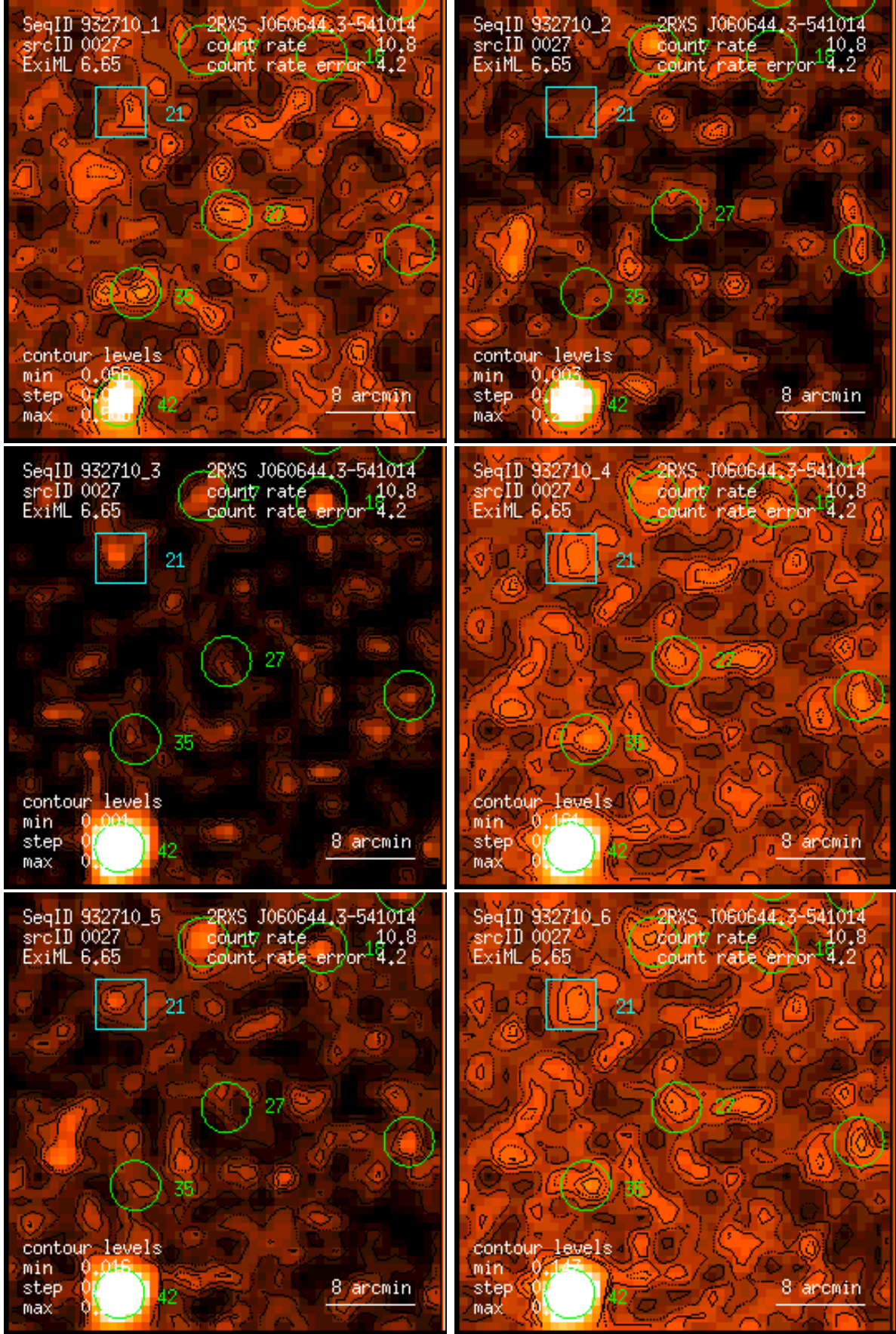
Figure 27: RASS 932710: detection 0027: band rate images, Gaussian filter: (1) PSPC channels 11 – 41, (2) 52 – 90, (3) 91 – 201, (4) 11 – 235, (5) 52 – 201, (6) 11 – 201. Broad band rates in counts/ks. Band rate contour levels in counts/ks/arcmin 2 .
