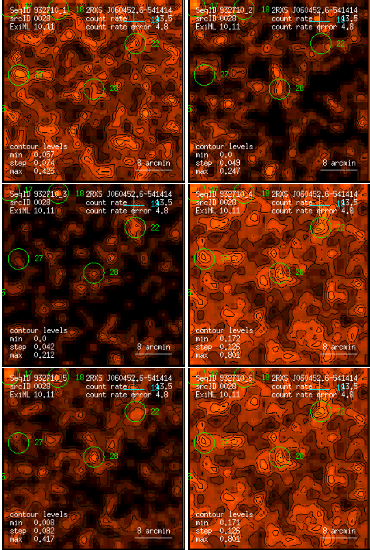
Figure 28: RASS 932710: detection 0028: band rate images, Gaussian filter: (1) PSPC channels 11 – 41, (2) 52 – 90, (3) 91 – 201, (4) 11 – 235, (5) 52 – 201, (6) 11 – 201. Broad band rates in counts/ks. Band rate contour levels in counts/ks/arcmin 2 .
