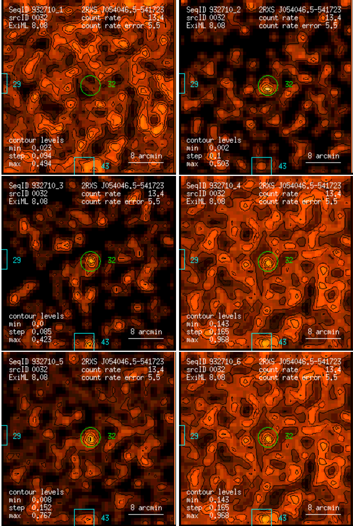
Figure 32: RASS 932710: detection 0032: band rate images, Gaussian filter: (1) PSPC channels 11 – 41, (2) 52 – 90, (3) 91 – 201, (4) 11 – 235, (5) 52 – 201, (6) 11 – 201. Broad band rates in counts/ks. Band rate contour levels in counts/ks/arcmin 2 .
