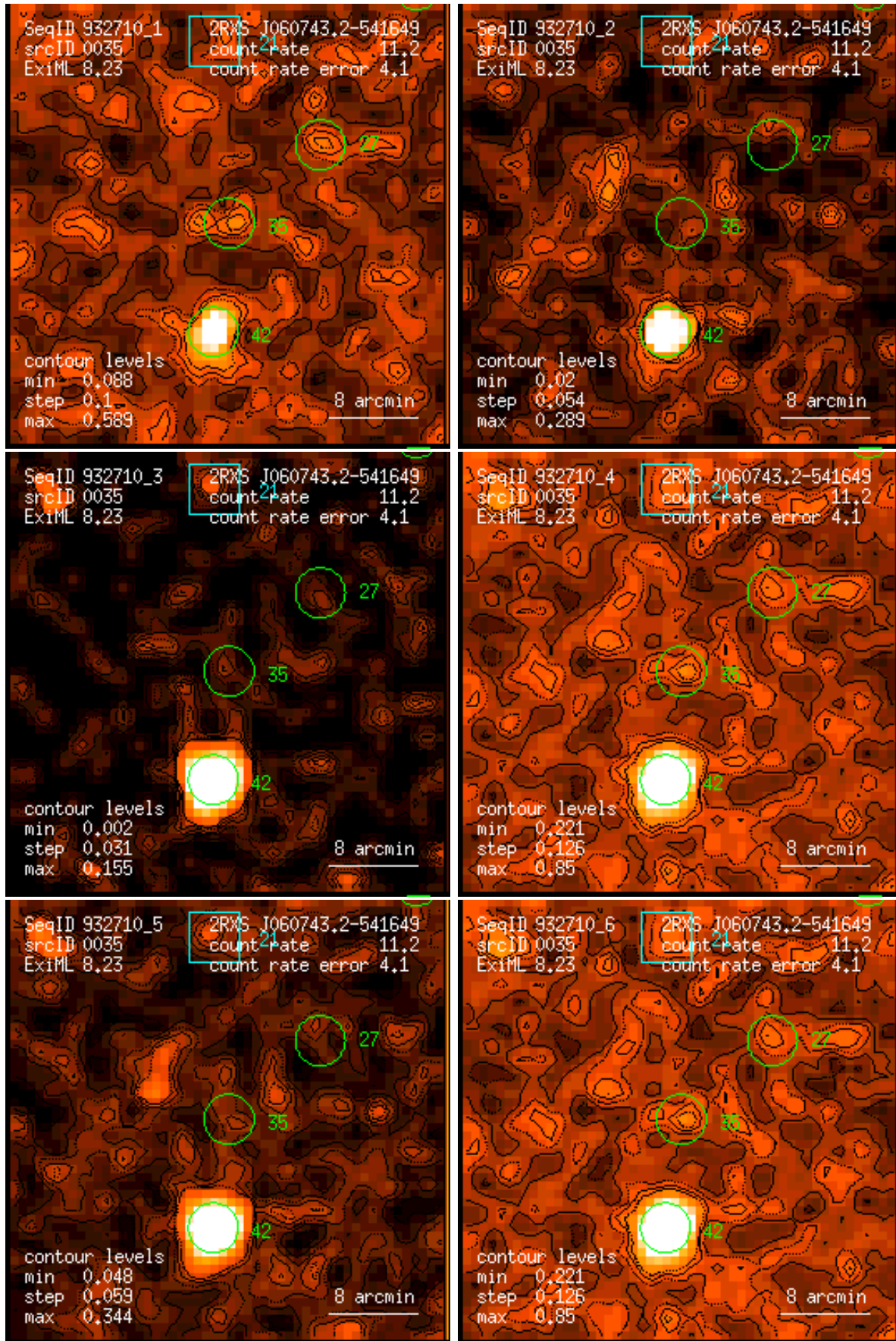
Figure 35: RASS 932710: detection 0035: band rate images, Gaussian filter: (1) PSPC channels 11 – 41, (2) 52 – 90, (3) 91 – 201, (4) 11 – 235, (5) 52 – 201, (6) 11 – 201. Broad band rates in counts/ks. Band rate contour levels in counts/ks/arcmin 2 .
