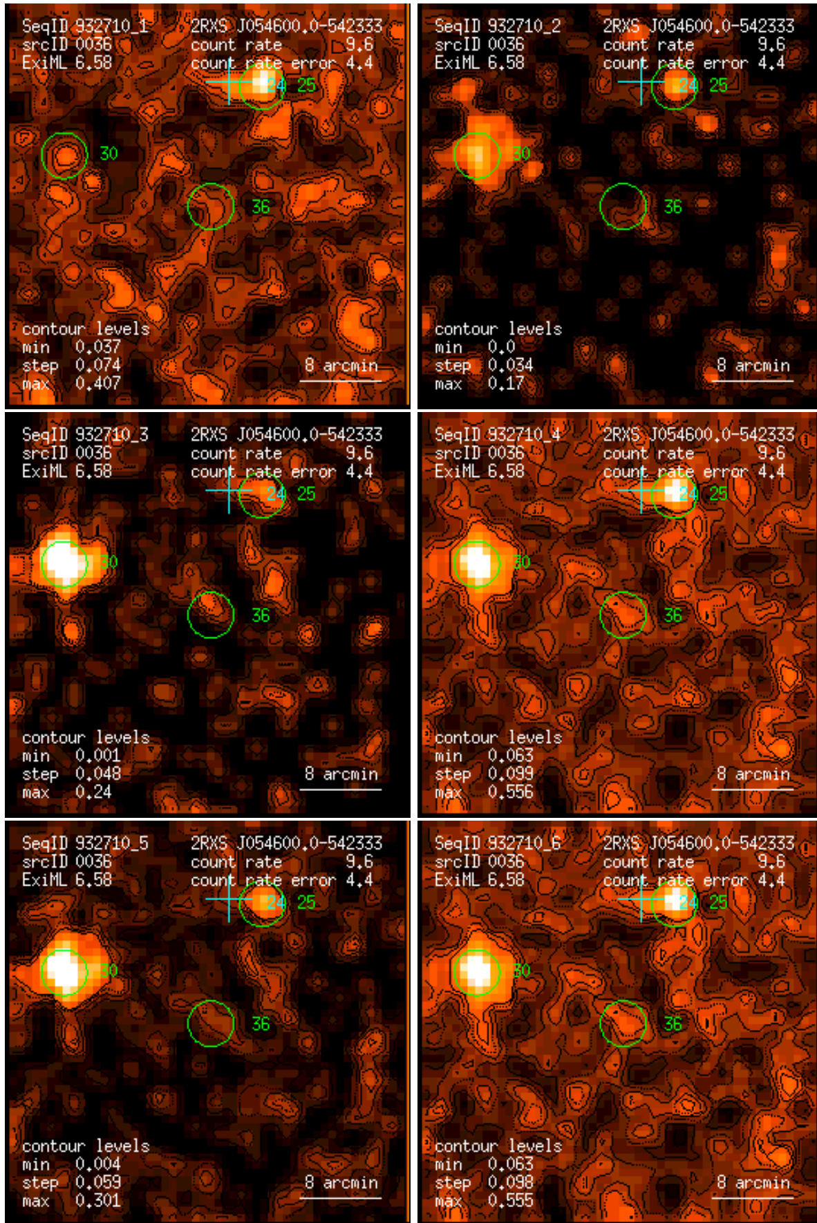
Figure 36: RASS 932710: detection 0036: band rate images, Gaussian filter: (1) PSPC channels 11 – 41, (2) 52 – 90, (3) 91 – 201, (4) 11 – 235, (5) 52 – 201, (6) 11 – 201. Broad band rates in counts/ks. Band rate contour levels in counts/ks/arcmin 2 .
