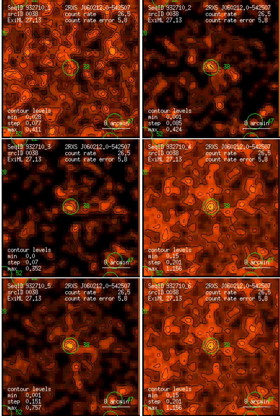
Figure 38: RASS 932710: detection 0038: band rate images, Gaussian filter: (1) PSPC channels 11 – 41, (2) 52 – 90, (3) 91 – 201, (4) 11 – 235, (5) 52 – 201, (6) 11 – 201. Broad band rates in counts/ks. Band rate contour levels in counts/ks/arcmin 2 .
