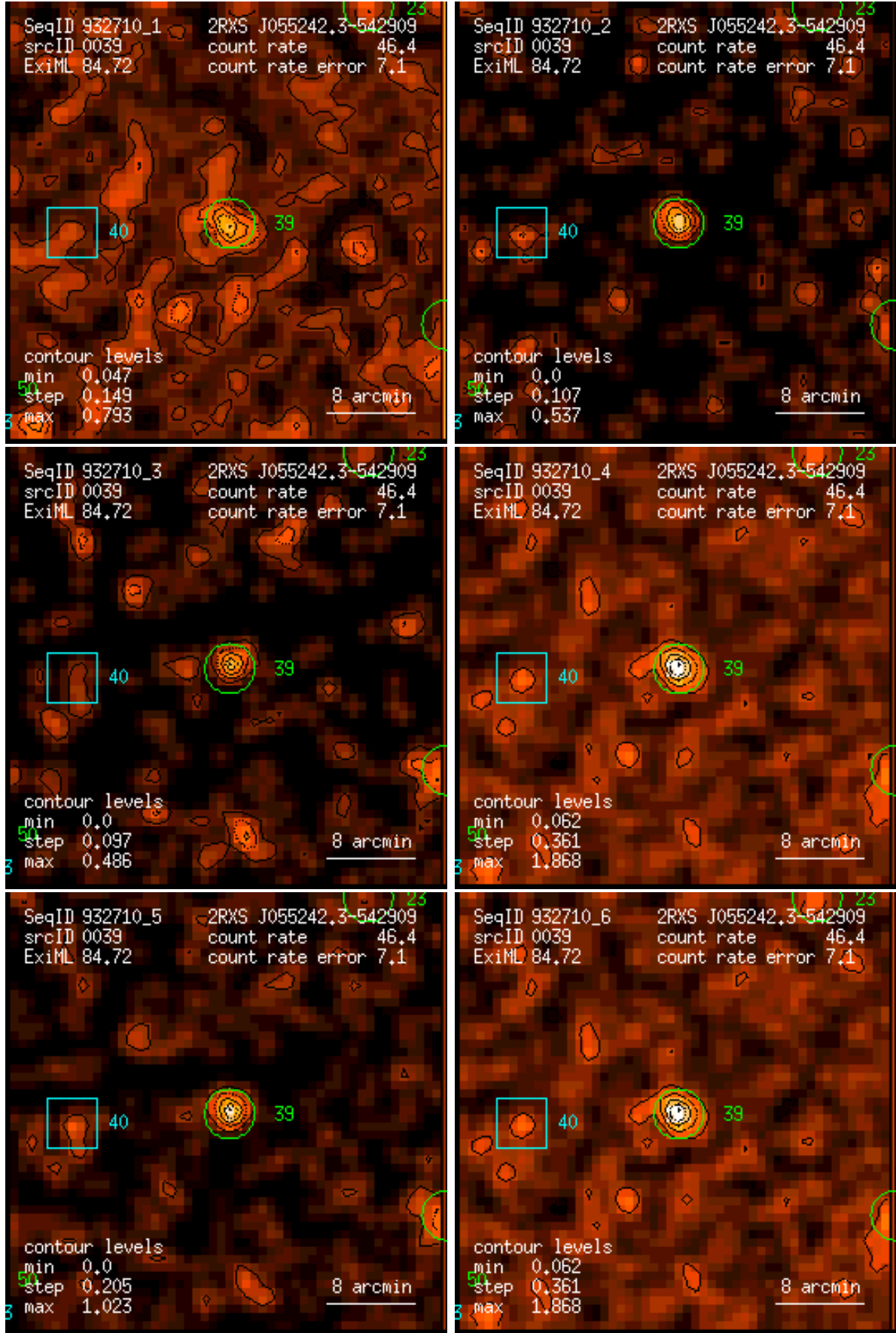
Figure 39: RASS 932710: detection 0039: band rate images, Gaussian filter: (1) PSPC channels 11 – 41, (2) 52 – 90, (3) 91 – 201, (4) 11 – 235, (5) 52 – 201, (6) 11 – 201. Broad band rates in counts/ks. Band rate contour levels in counts/ks/arcmin 2 .
