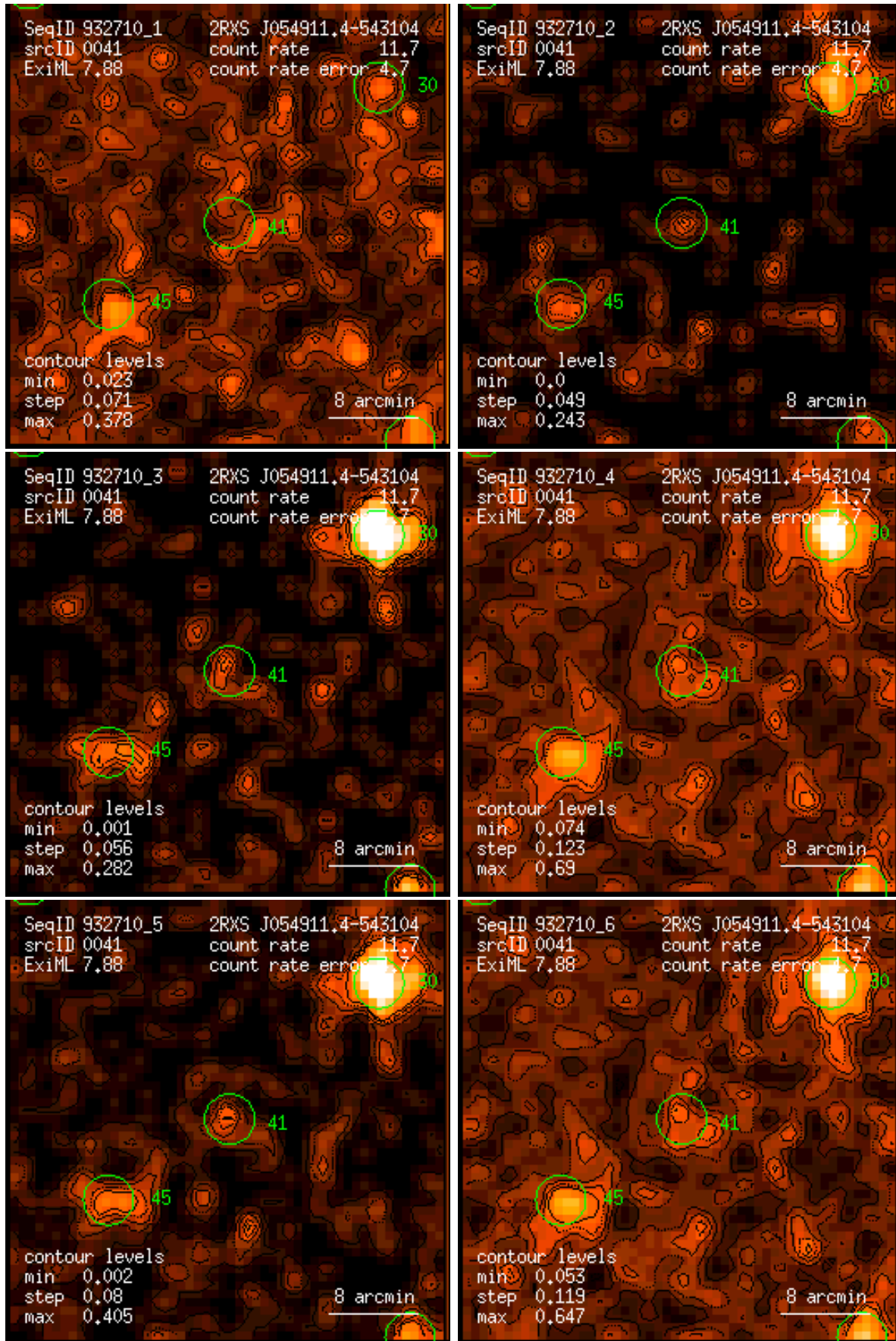
Figure 41: RASS 932710: detection 0041: band rate images, Gaussian filter: (1) PSPC channels 11 – 41, (2) 52 – 90, (3) 91 – 201, (4) 11 – 235, (5) 52 – 201, (6) 11 – 201. Broad band rates in counts/ks. Band rate contour levels in counts/ks/arcmin 2 .
