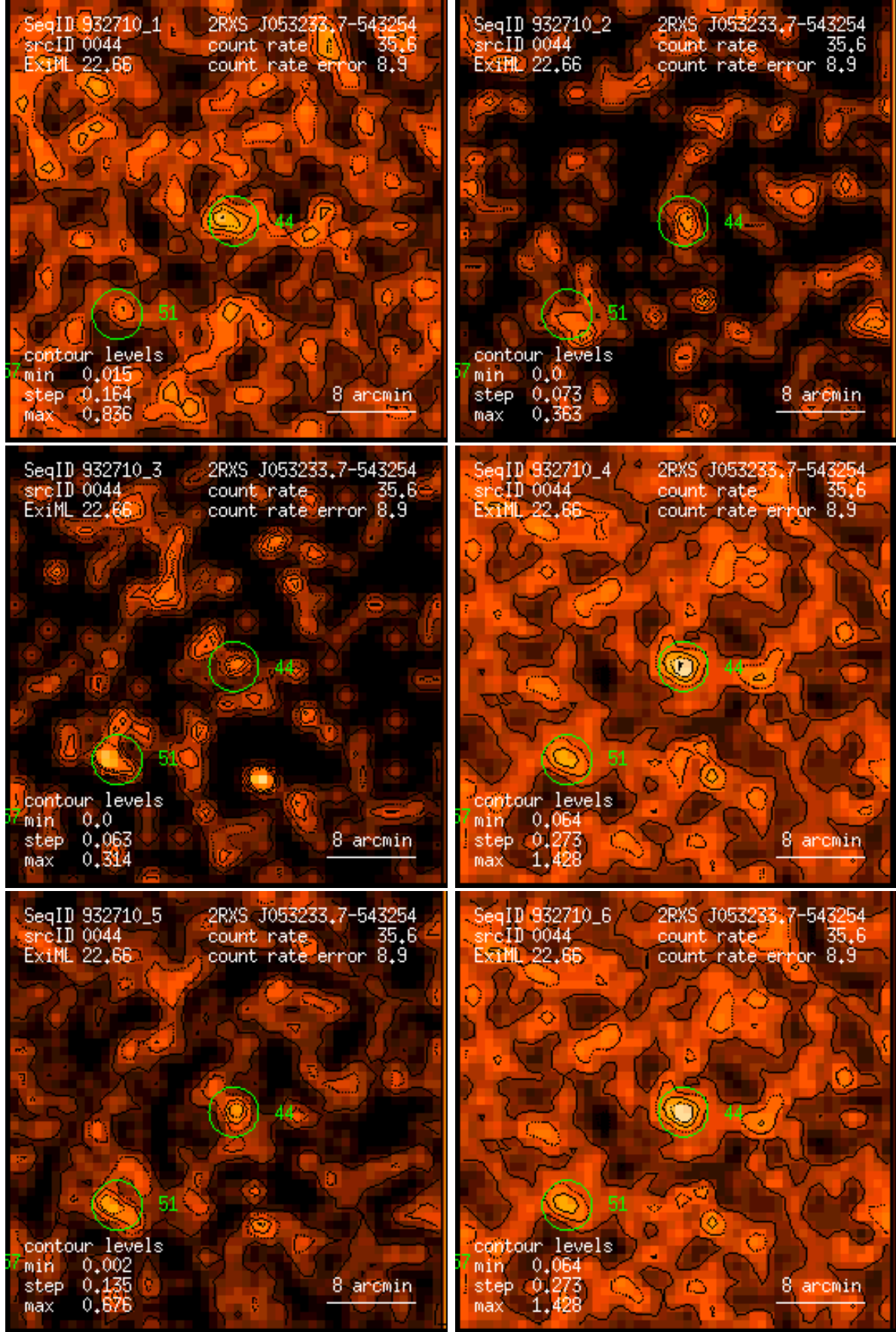
Figure 44: RASS 932710: detection 0044: band rate images, Gaussian filter: (1) PSPC channels 11 – 41, (2) 52 – 90, (3) 91 – 201, (4) 11 – 235, (5) 52 – 201, (6) 11 – 201. Broad band rates in counts/ks. Band rate contour levels in counts/ks/arcmin 2 .
