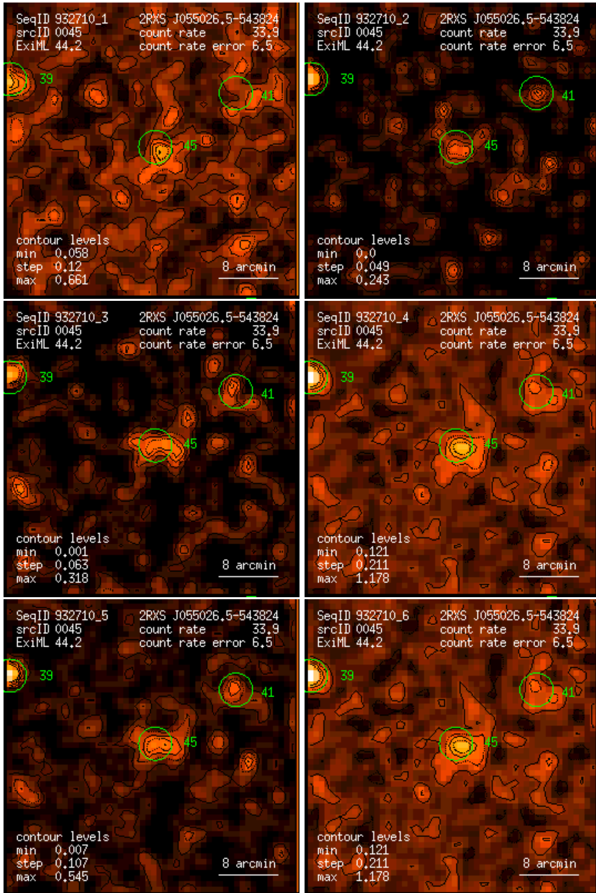
Figure 45: RASS 932710: detection 0045: band rate images, Gaussian filter: (1) PSPC channels 11 – 41, (2) 52 – 90, (3) 91 – 201, (4) 11 – 235, (5) 52 – 201, (6) 11 – 201. Broad band rates in counts/ks. Band rate contour levels in counts/ks/arcmin 2 .
