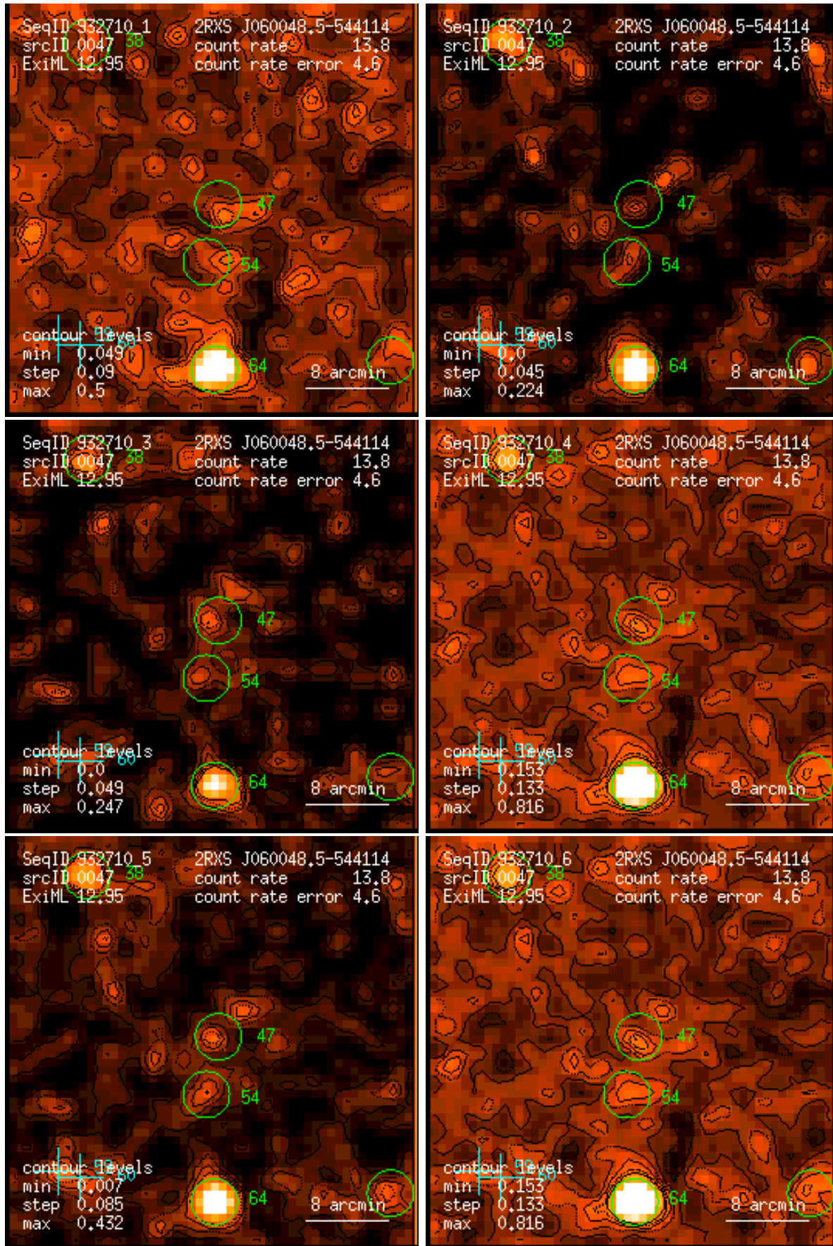
Figure 47: RASS 932710: detection 0047: band rate images, Gaussian filter: (1) PSPC channels 11 – 41, (2) 52 – 90, (3) 91 – 201, (4) 11 – 235, (5) 52 – 201, (6) 11 – 201. Broad band rates in counts/ks. Band rate contour levels in counts/ks/arcmin 2 .
