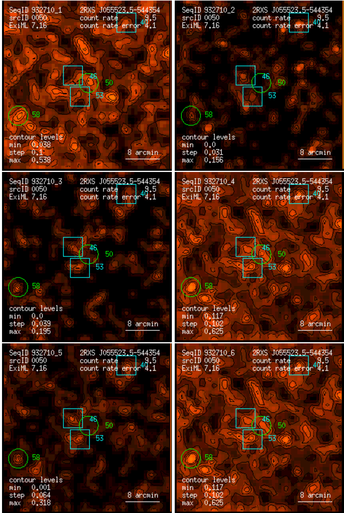
Figure 50: RASS 932710: detection 0050: band rate images, Gaussian filter: (1) PSPC channels 11 – 41, (2) 52 – 90, (3) 91 – 201, (4) 11 – 235, (5) 52 – 201, (6) 11 – 201. Broad band rates in counts/ks. Band rate contour levels in counts/ks/arcmin 2 .
