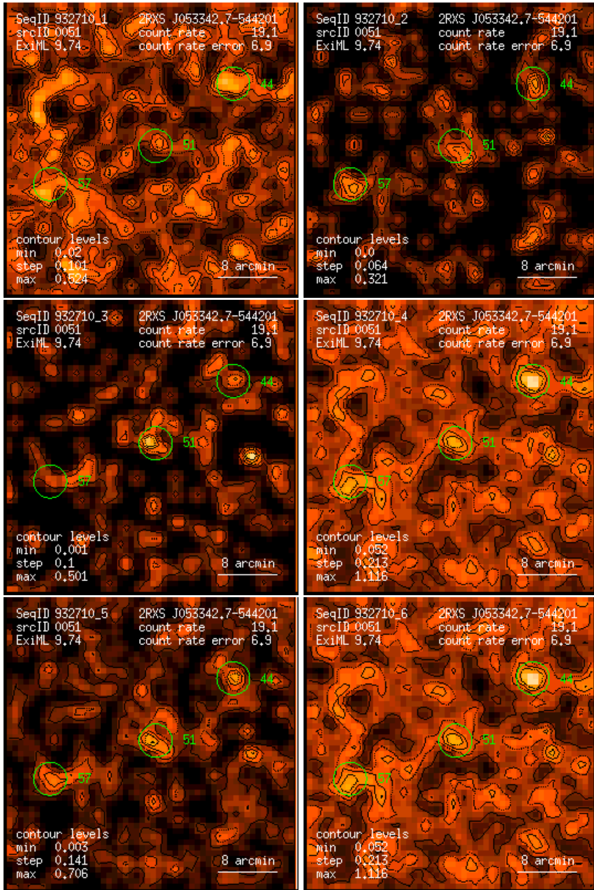
Figure 51: RASS 932710: detection 0051: band rate images, Gaussian filter: (1) PSPC channels 11 – 41, (2) 52 – 90, (3) 91 – 201, (4) 11 – 235, (5) 52 – 201, (6) 11 – 201. Broad band rates in counts/ks. Band rate contour levels in counts/ks/arcmin 2 .
