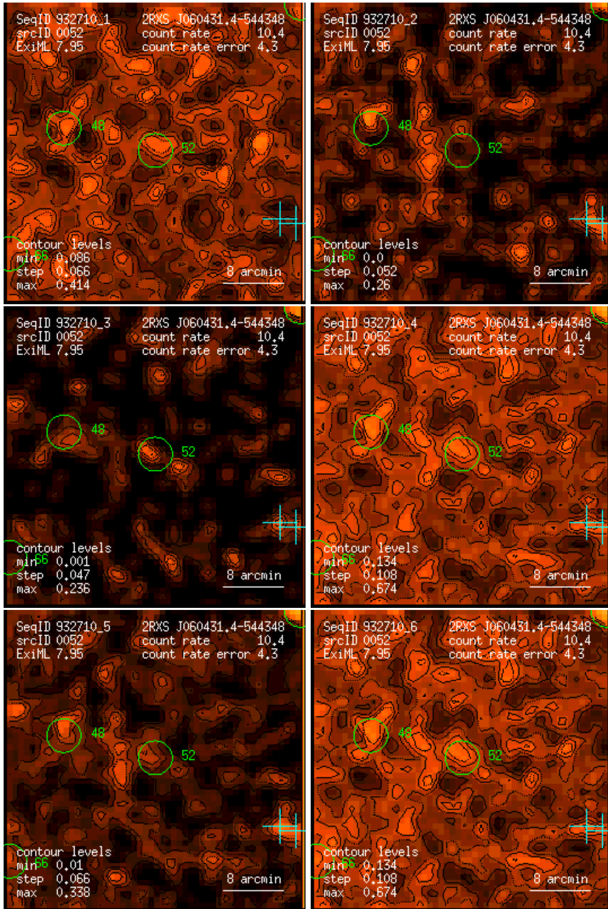
Figure 52: RASS 932710: detection 0052: band rate images, Gaussian filter: (1) PSPC channels 11 – 41, (2) 52 – 90, (3) 91 – 201, (4) 11 – 235, (5) 52 – 201, (6) 11 – 201. Broad band rates in counts/ks. Band rate contour levels in counts/ks/arcmin 2 .
