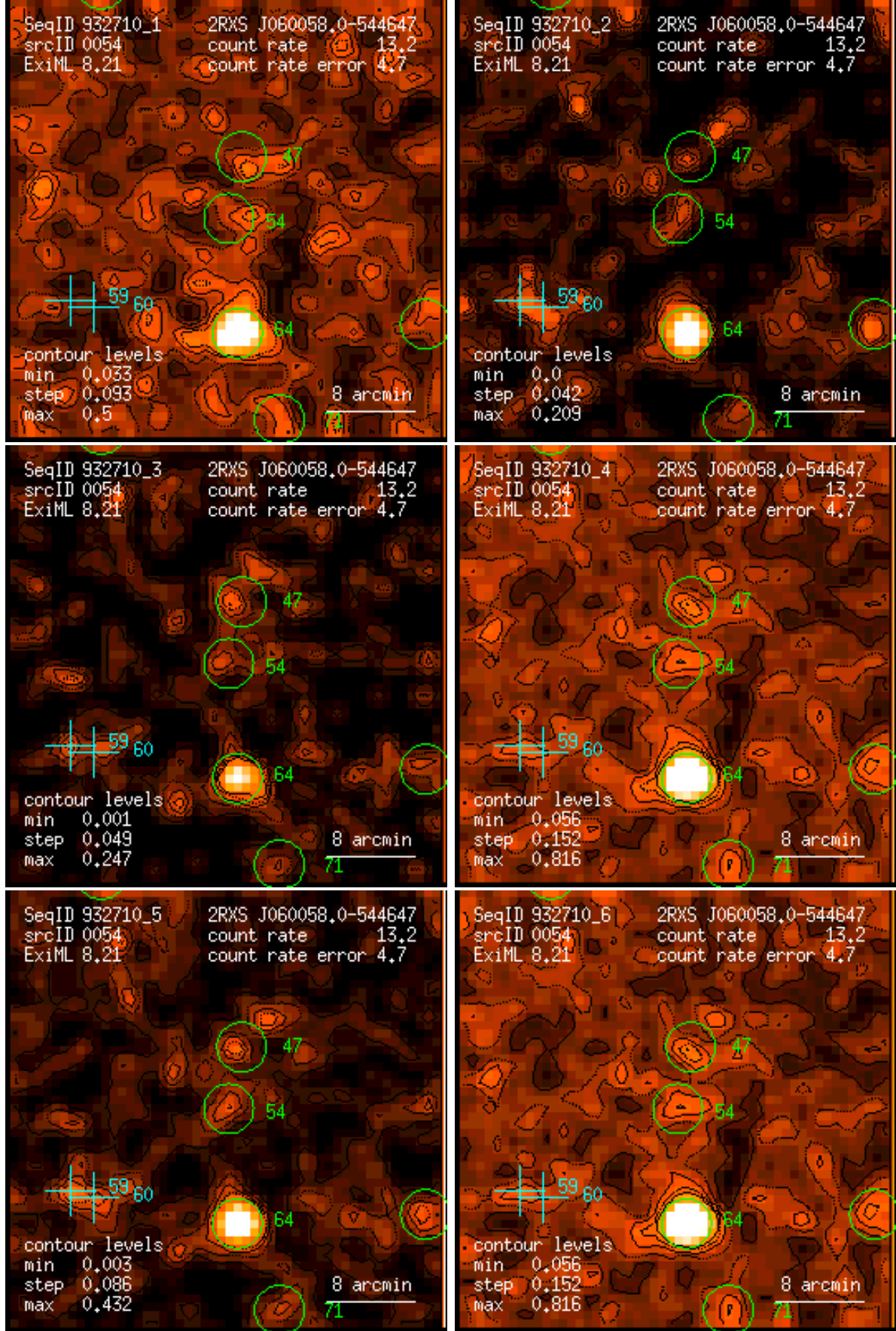
Figure 54: RASS 932710: detection 0054: band rate images, Gaussian filter: (1) PSPC channels 11 – 41, (2) 52 – 90, (3) 91 – 201, (4) 11 – 235, (5) 52 – 201, (6) 11 – 201. Broad band rates in counts/ks. Band rate contour levels in counts/ks/arcmin 2 .
