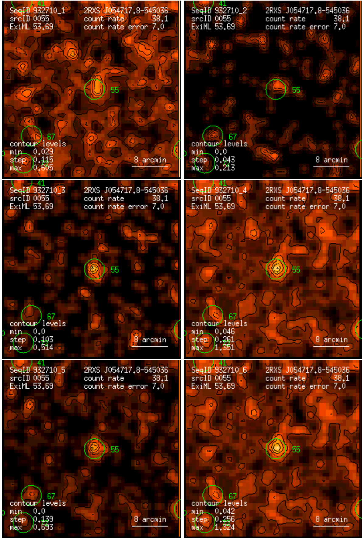
Figure 55: RASS 932710: detection 0055: band rate images, Gaussian filter: (1) PSPC channels 11 – 41, (2) 52 – 90, (3) 91 – 201, (4) 11 – 235, (5) 52 – 201, (6) 11 – 201. Broad band rates in counts/ks. Band rate contour levels in counts/ks/arcmin 2 .
