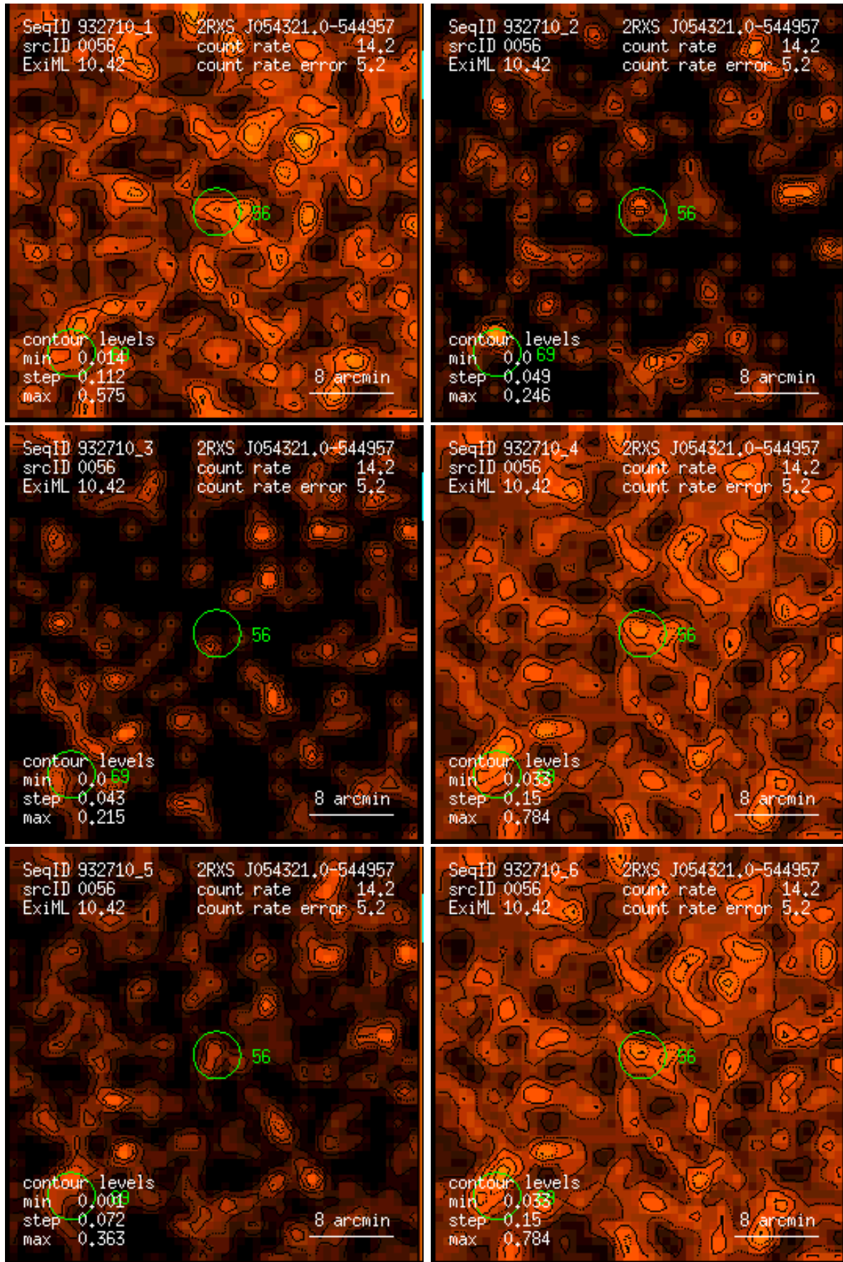
Figure 56: RASS 932710: detection 0056: band rate images, Gaussian filter: (1) PSPC channels 11 – 41, (2) 52 – 90, (3) 91 – 201, (4) 11 – 235, (5) 52 – 201, (6) 11 – 201. Broad band rates in counts/ks. Band rate contour levels in counts/ks/arcmin 2 .
