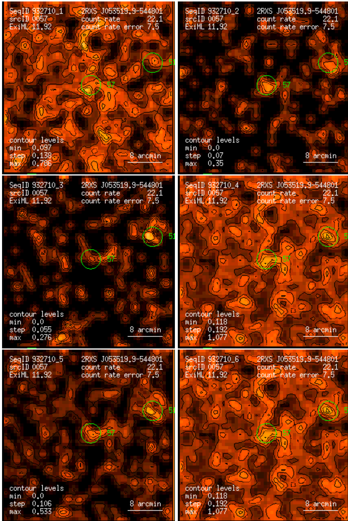
Figure 57: RASS 932710: detection 0057: band rate images, Gaussian filter: (1) PSPC channels 11 – 41, (2) 52 – 90, (3) 91 – 201, (4) 11 – 235, (5) 52 – 201, (6) 11 – 201. Broad band rates in counts/ks. Band rate contour levels in counts/ks/arcmin 2 .
