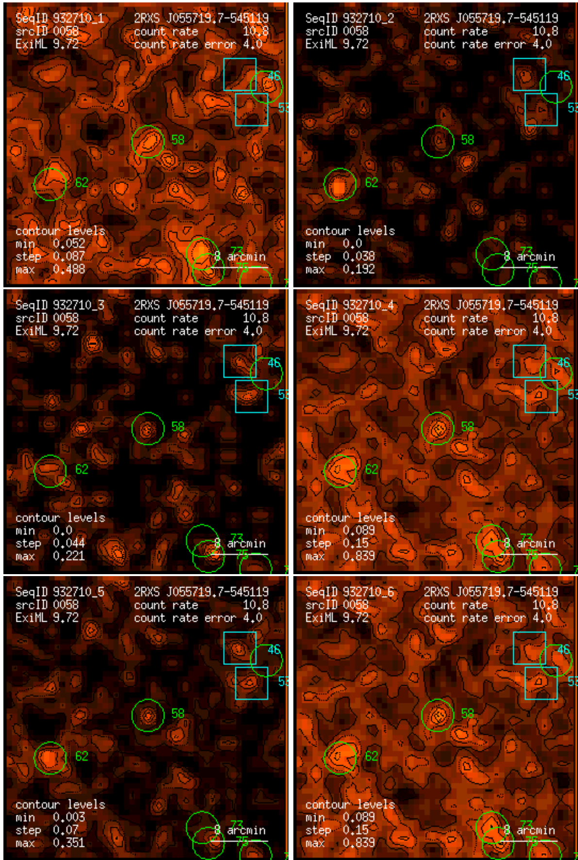
Figure 58: RASS 932710: detection 0058: band rate images, Gaussian filter: (1) PSPC channels 11 – 41, (2) 52 – 90, (3) 91 – 201, (4) 11 – 235, (5) 52 – 201, (6) 11 – 201. Broad band rates in counts/ks. Band rate contour levels in counts/ks/arcmin 2 .
