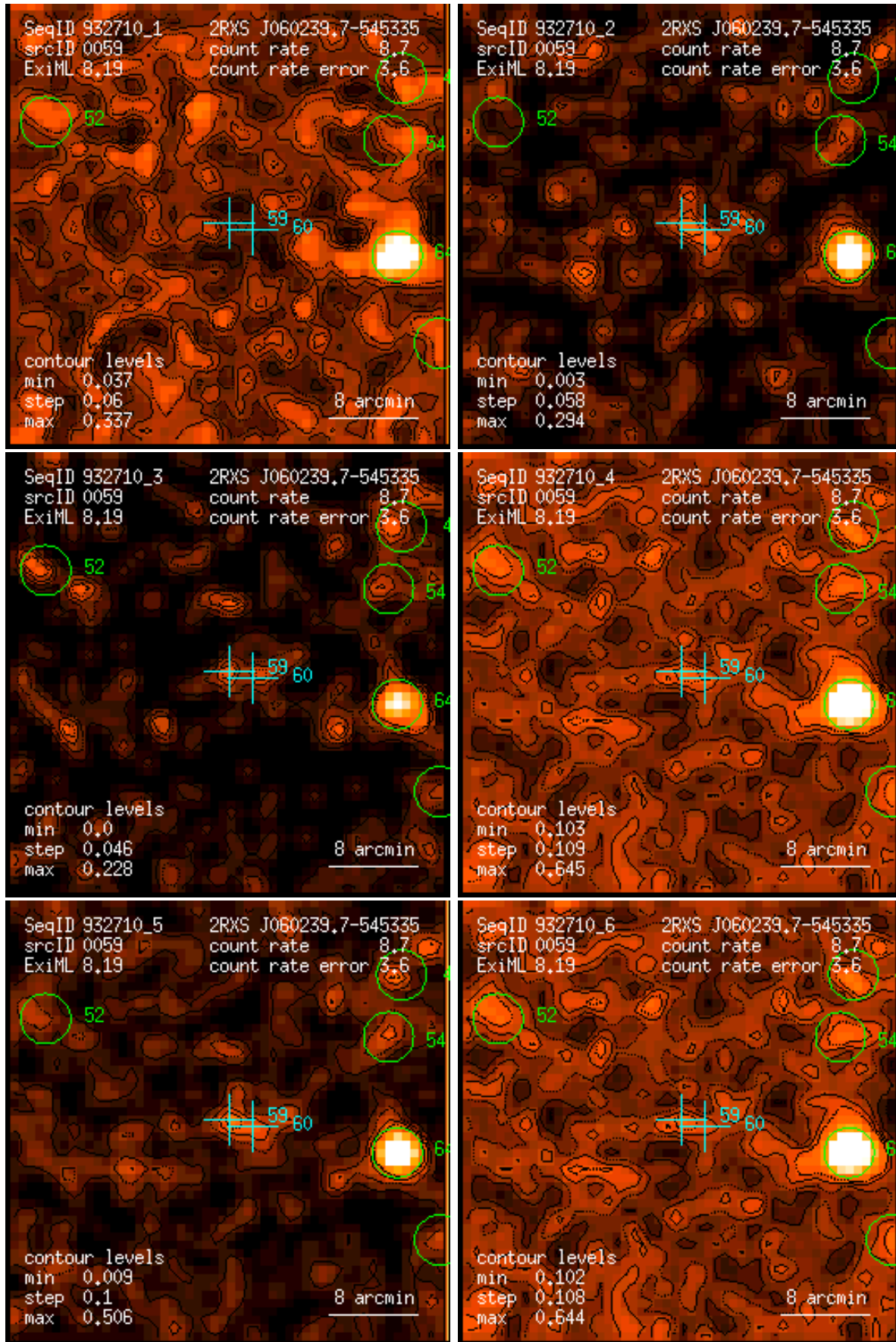
Figure 59: RASS 932710: detection 0059: band rate images, Gaussian filter: (1) PSPC channels 11 – 41, (2) 52 – 90, (3) 91 – 201, (4) 11 – 235, (5) 52 – 201, (6) 11 – 201. Broad band rates in counts/ks. Band rate contour levels in counts/ks/arcmin 2 .
