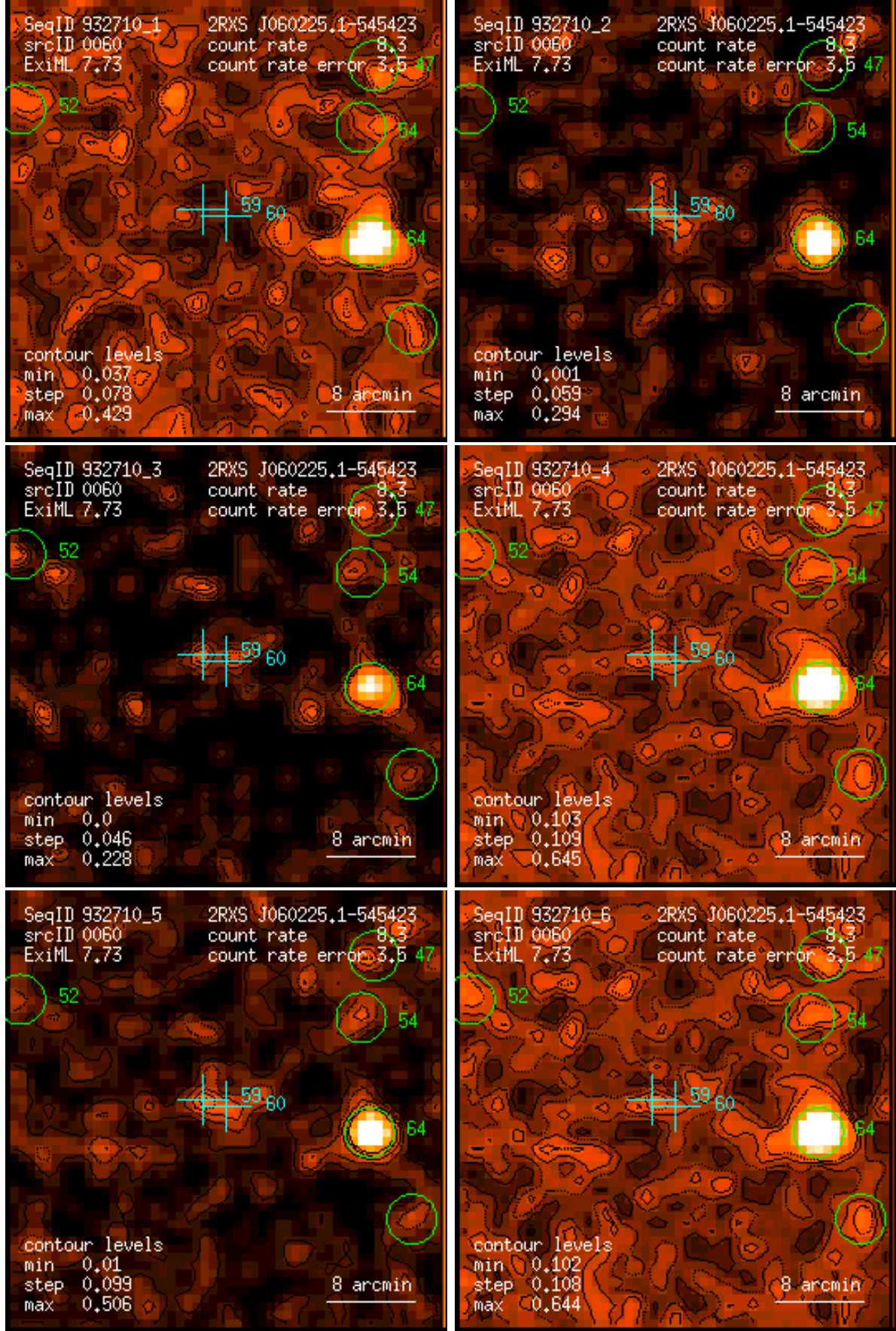
Figure 60: RASS 932710: detection 0060: band rate images, Gaussian filter: (1) PSPC channels 11 – 41, (2) 52 – 90, (3) 91 – 201, (4) 11 – 235, (5) 52 – 201, (6) 11 – 201. Broad band rates in counts/ks. Band rate contour levels in counts/ks/arcmin 2 .
