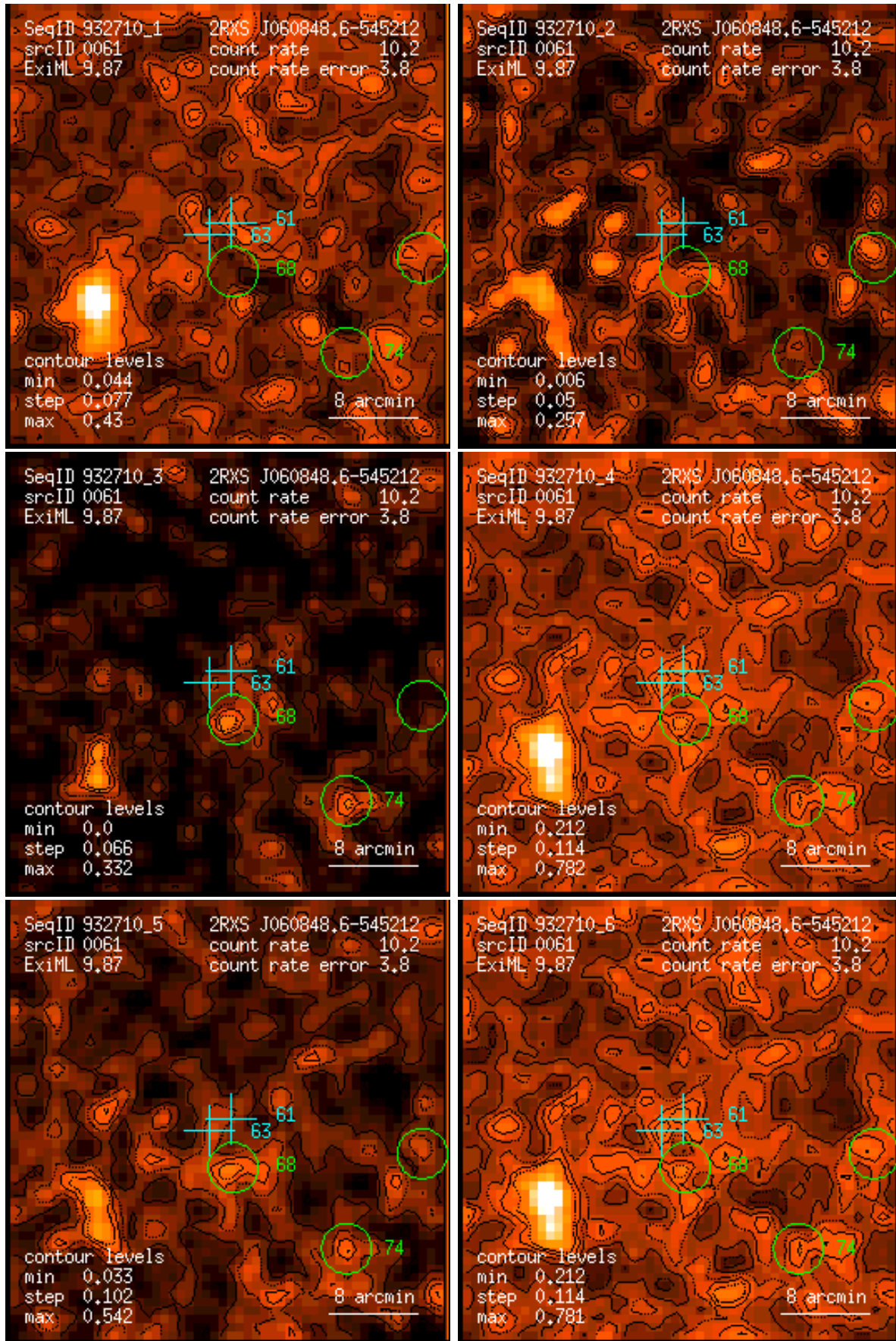
Figure 61: RASS 932710: detection 0061: band rate images, Gaussian filter: (1) PSPC channels 11 – 41, (2) 52 – 90, (3) 91 – 201, (4) 11 – 235, (5) 52 – 201, (6) 11 – 201. Broad band rates in counts/ks. Band rate contour levels in counts/ks/arcmin 2 .
