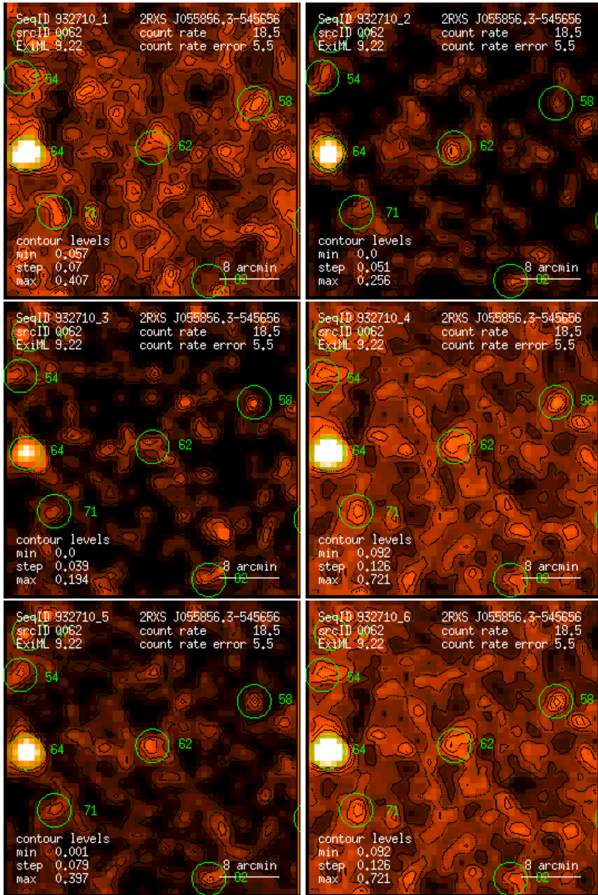
Figure 62: RASS 932710: detection 0062: band rate images, Gaussian filter: (1) PSPC channels 11 – 41, (2) 52 – 90, (3) 91 – 201, (4) 11 – 235, (5) 52 – 201, (6) 11 – 201. Broad band rates in counts/ks. Band rate contour levels in counts/ks/arcmin 2 .
