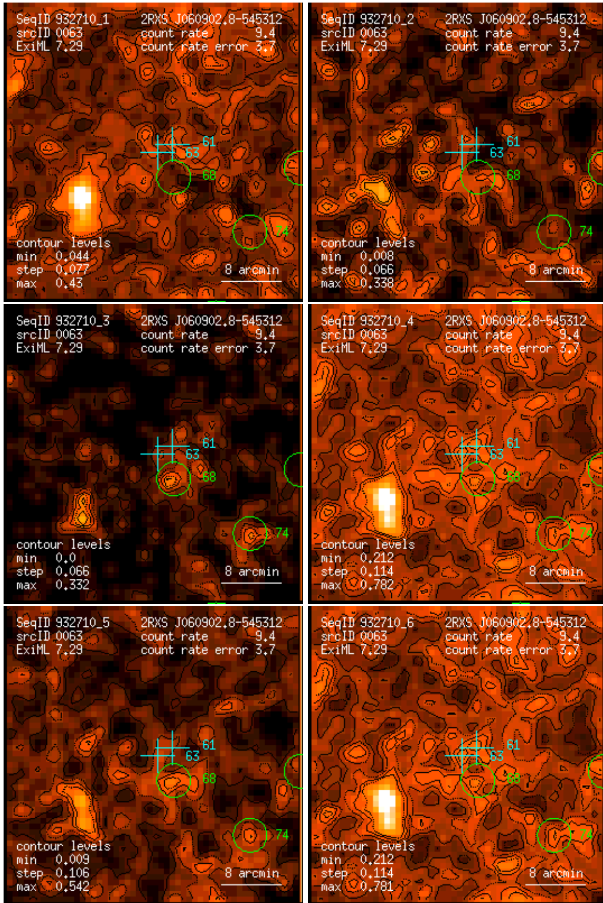
Figure 63: RASS 932710: detection 0063: band rate images, Gaussian filter: (1) PSPC channels 11 – 41, (2) 52 – 90, (3) 91 – 201, (4) 11 – 235, (5) 52 – 201, (6) 11 – 201. Broad band rates in counts/ks. Band rate contour levels in counts/ks/arcmin 2 .
