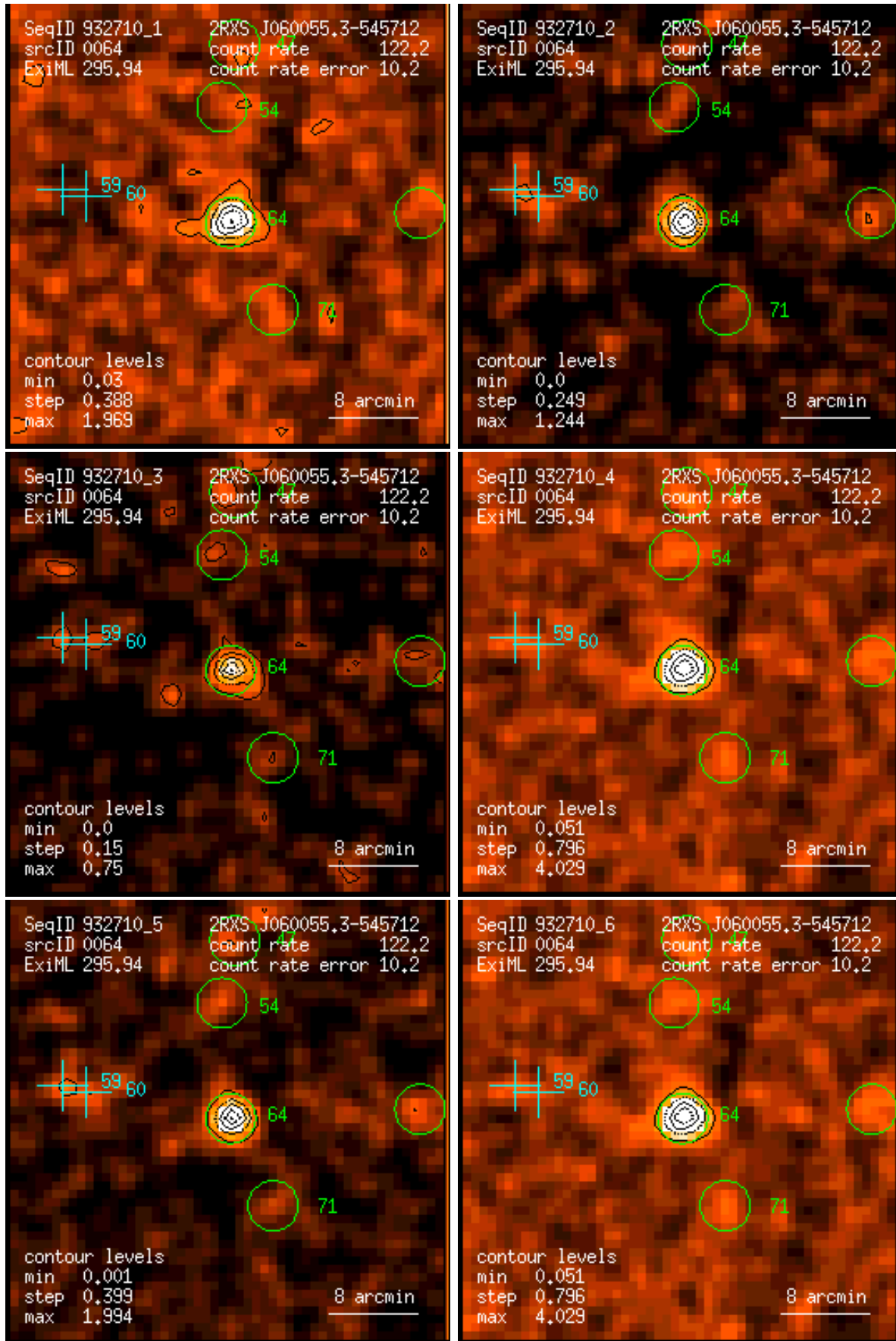
Figure 64: RASS 932710: detection 0064: band rate images, Gaussian filter: (1) PSPC channels 11 – 41, (2) 52 – 90, (3) 91 – 201, (4) 11 – 235, (5) 52 – 201, (6) 11 – 201. Broad band rates in counts/ks. Band rate contour levels in counts/ks/arcmin 2 .
