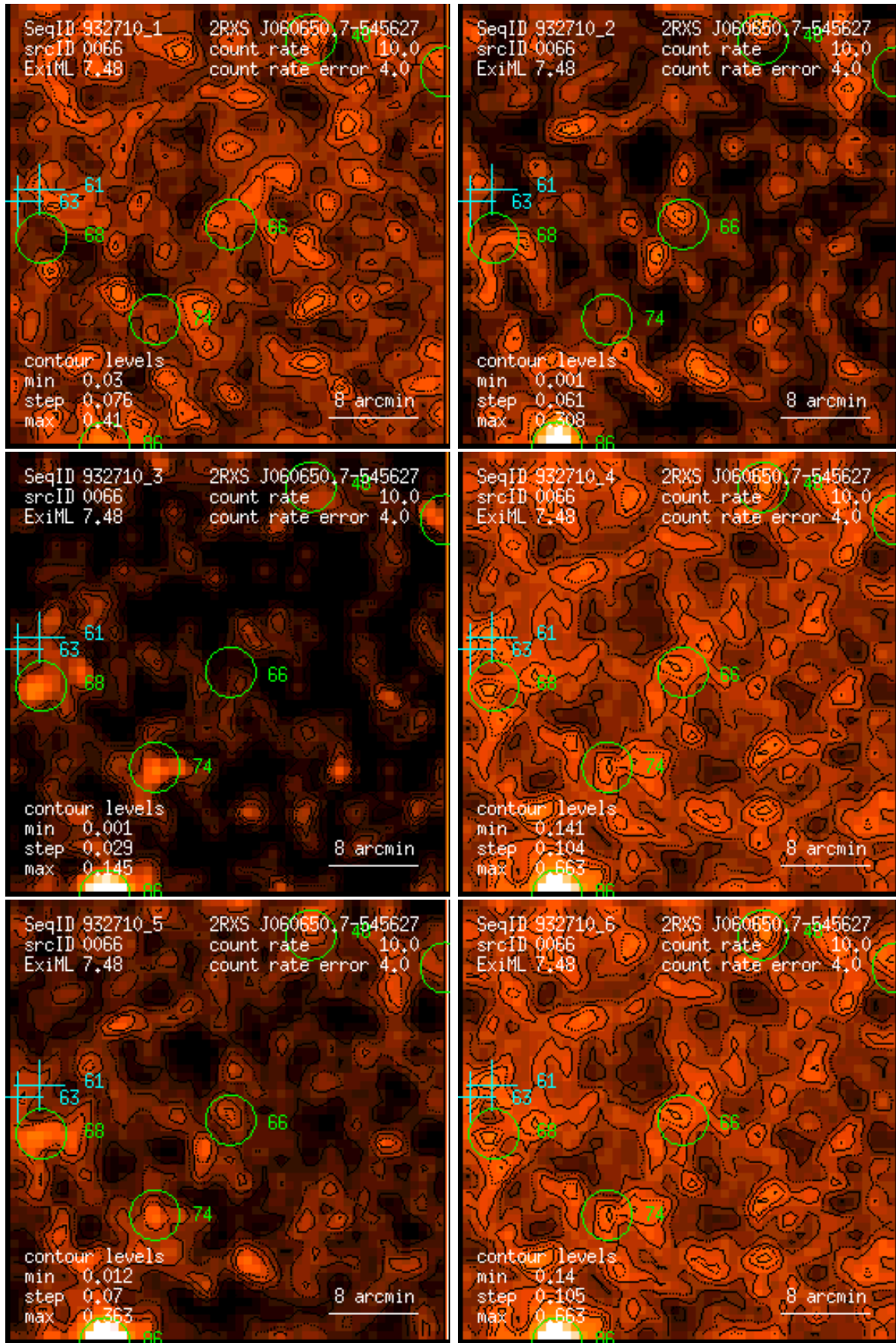
Figure 66: RASS 932710: detection 0066: band rate images, Gaussian filter: (1) PSPC channels 11 – 41, (2) 52 – 90, (3) 91 – 201, (4) 11 – 235, (5) 52 – 201, (6) 11 – 201. Broad band rates in counts/ks. Band rate contour levels in counts/ks/arcmin 2 .
