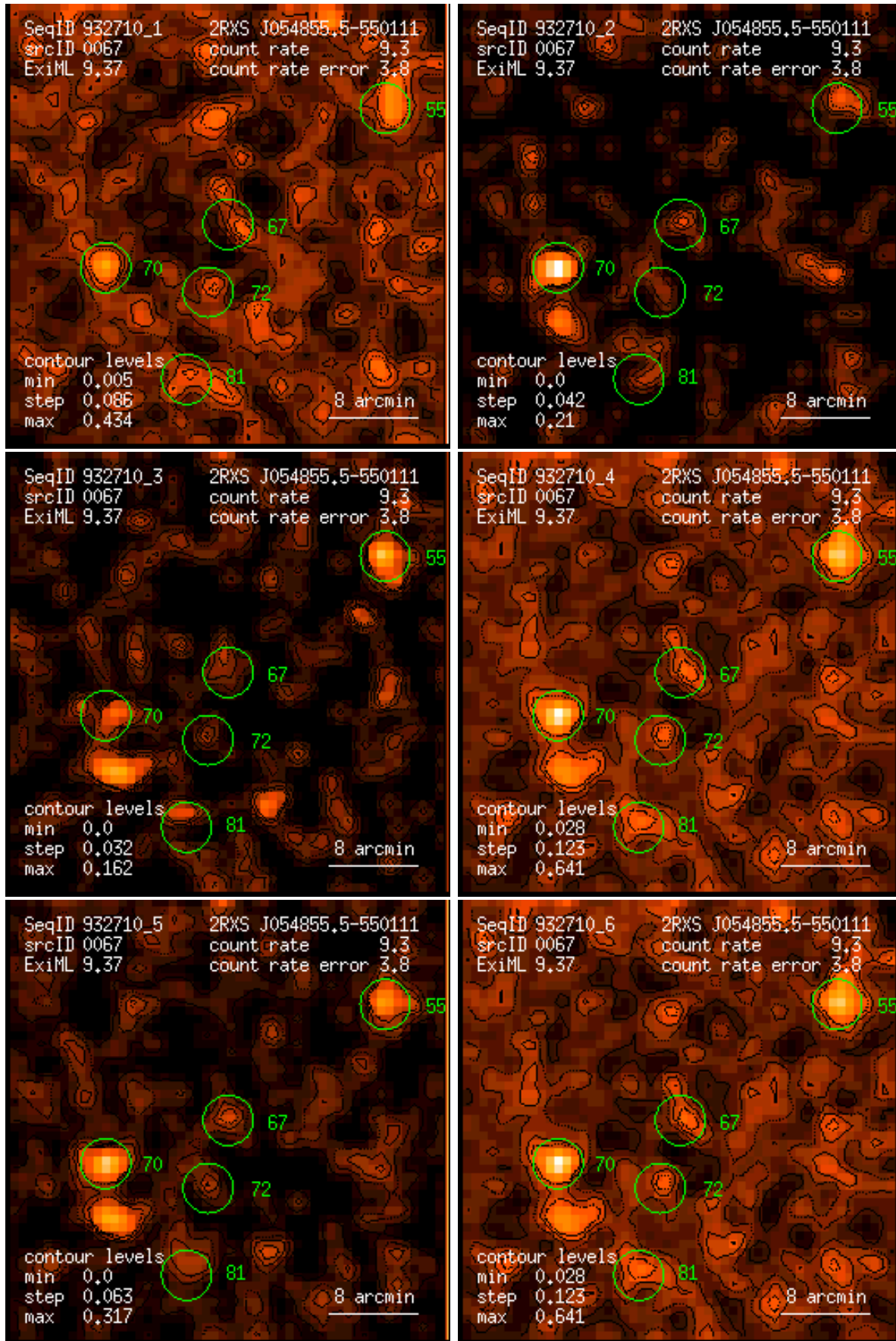
Figure 67: RASS 932710: detection 0067: band rate images, Gaussian filter: (1) PSPC channels 11 – 41, (2) 52 – 90, (3) 91 – 201, (4) 11 – 235, (5) 52 – 201, (6) 11 – 201. Broad band rates in counts/ks. Band rate contour levels in counts/ks/arcmin 2 .
