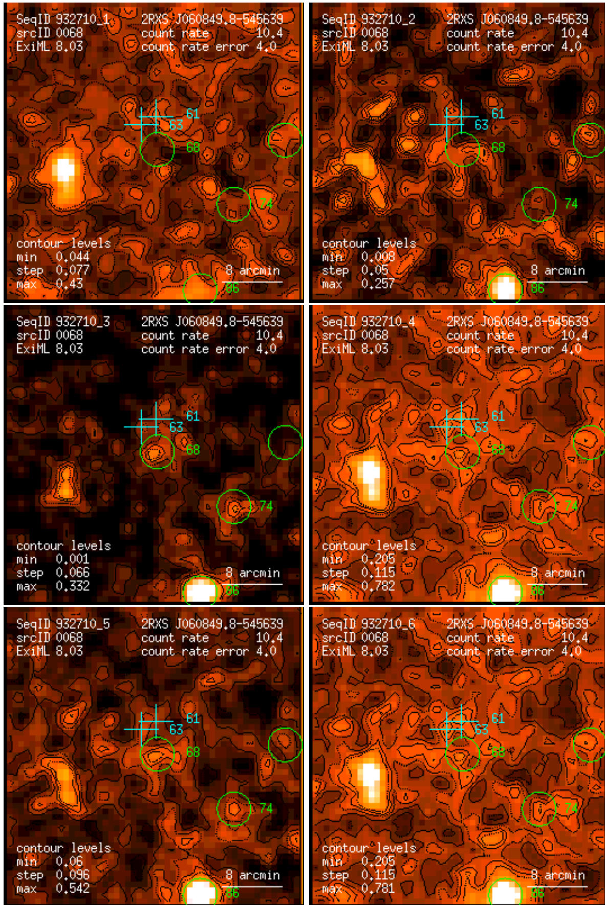
Figure 68: RASS 932710: detection 0068: band rate images, Gaussian filter: (1) PSPC channels 11 – 41, (2) 52 – 90, (3) 91 – 201, (4) 11 – 235, (5) 52 – 201, (6) 11 – 201. Broad band rates in counts/ks. Band rate contour levels in counts/ks/arcmin 2 .
