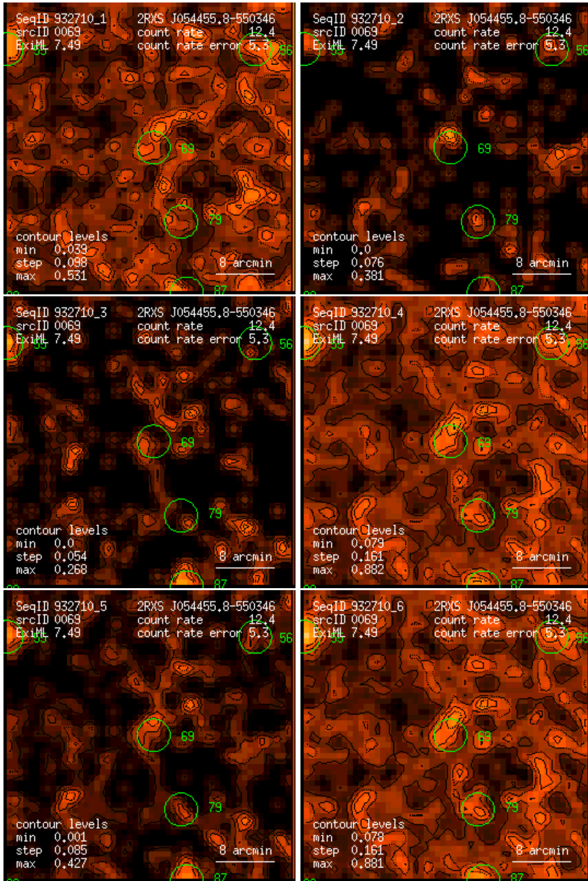
Figure 69: RASS 932710: detection 0069: band rate images, Gaussian filter: (1) PSPC channels 11 – 41, (2) 52 – 90, (3) 91 – 201, (4) 11 – 235, (5) 52 – 201, (6) 11 – 201. Broad band rates in counts/ks. Band rate contour levels in counts/ks/arcmin 2 .
