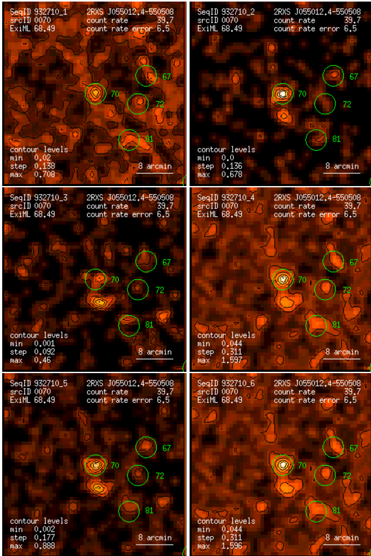
Figure 70: RASS 932710: detection 0070: band rate images, Gaussian filter: (1) PSPC channels 11 – 41, (2) 52 – 90, (3) 91 – 201, (4) 11 – 235, (5) 52 – 201, (6) 11 – 201. Broad band rates in counts/ks. Band rate contour levels in counts/ks/arcmin 2 .
