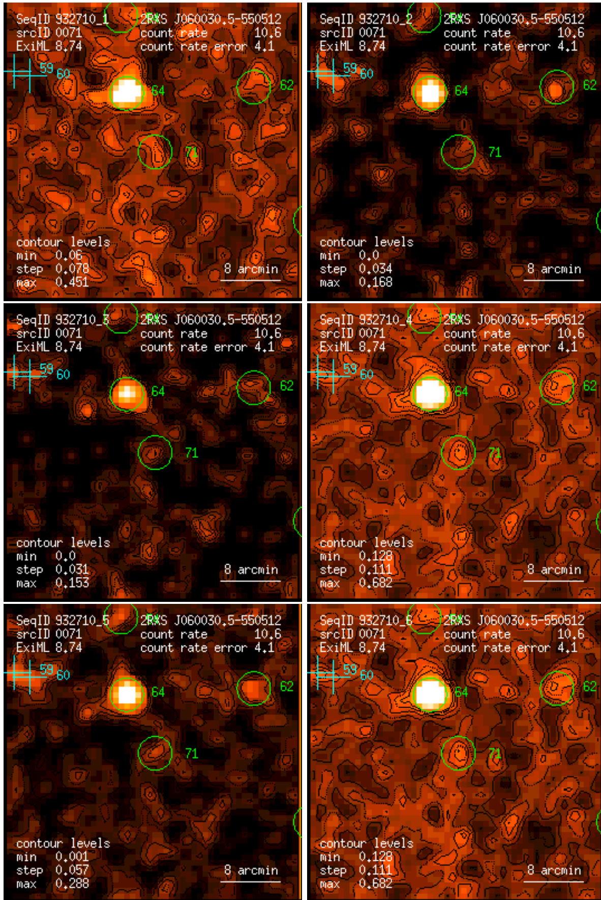
Figure 71: RASS 932710: detection 0071: band rate images, Gaussian filter: (1) PSPC channels 11 – 41, (2) 52 – 90, (3) 91 – 201, (4) 11 – 235, (5) 52 – 201, (6) 11 – 201. Broad band rates in counts/ks. Band rate contour levels in counts/ks/arcmin 2 .
