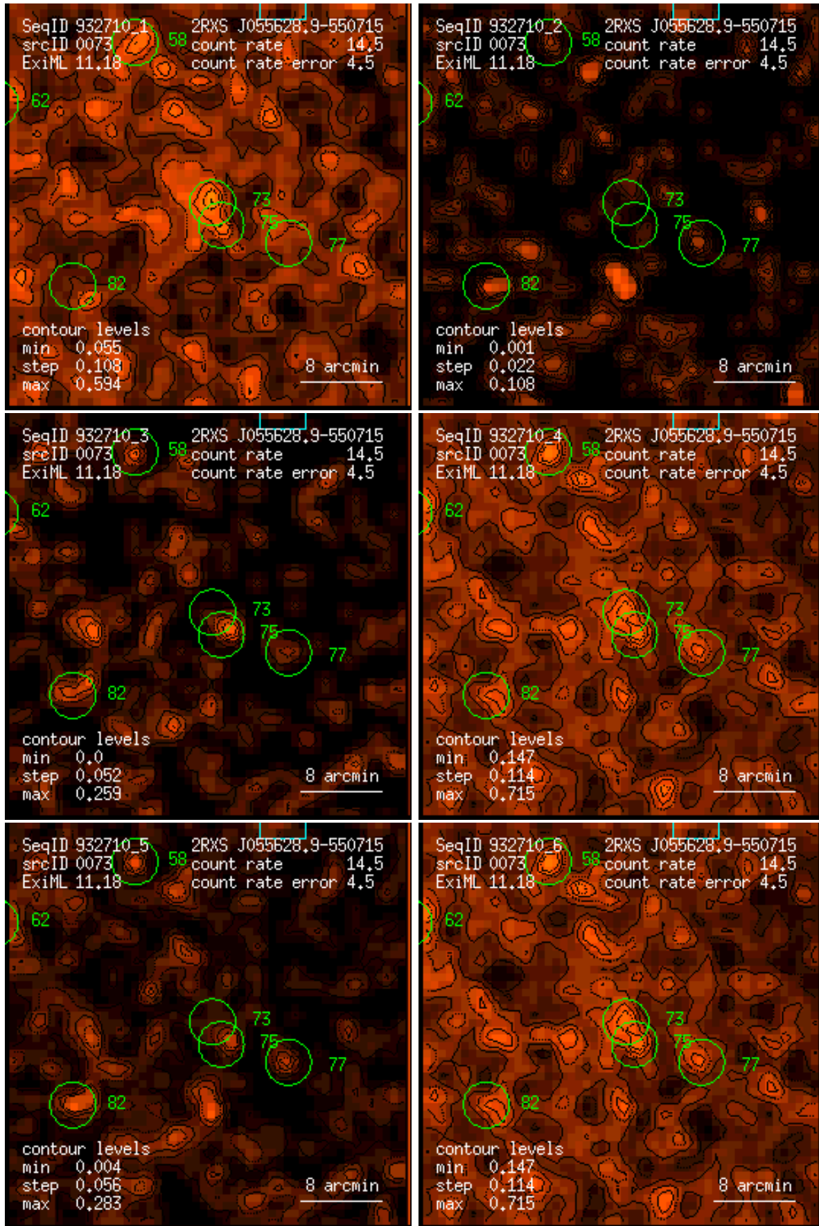
Figure 73: RASS 932710: detection 0073: band rate images, Gaussian filter: (1) PSPC channels 11 – 41, (2) 52 – 90, (3) 91 – 201, (4) 11 – 235, (5) 52 – 201, (6) 11 – 201. Broad band rates in counts/ks. Band rate contour levels in counts/ks/arcmin 2 .
